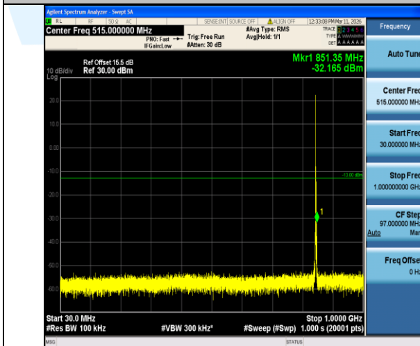
Band5-3MHz-QPSK-20635-1RB#0-30~1000-PASS
