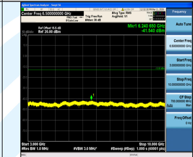
Band5-3MHz-QPSK-20525-1RB#0-3000~10000-PASS
