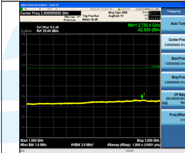
Band5-3MHz-QPSK-20525-1RB#0-1000~3000-PASS
