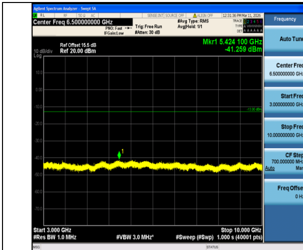
Band5-3MHz-QPSK-20415-1RB#0-3000~10000-PASS
