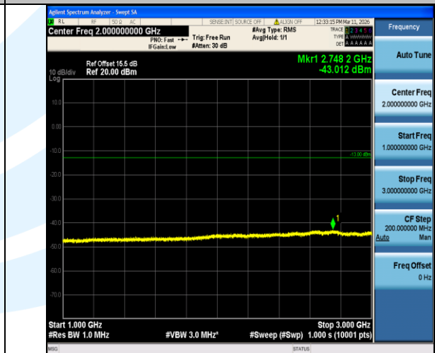
Band5-3MHz-QPSK-20635-1RB#0-1000~3000-PASS
