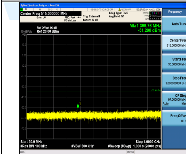
Band38-5MHz-16QAM-37775-1RB#0-30~1000-PASS
