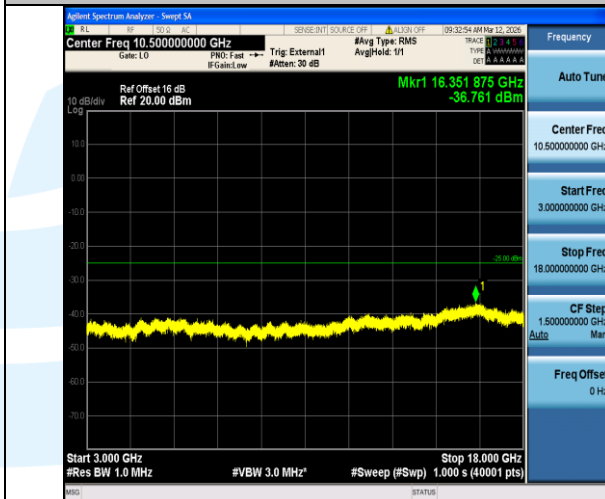
Band38-5MHz-QPSK-38225-1RB#0-3000~18000-PASS
