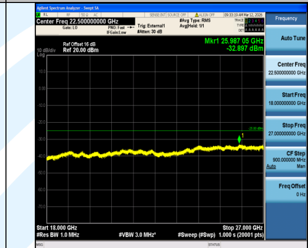
Band38-5MHz-QPSK-38225-1RB#0-18000~27000-PASS
