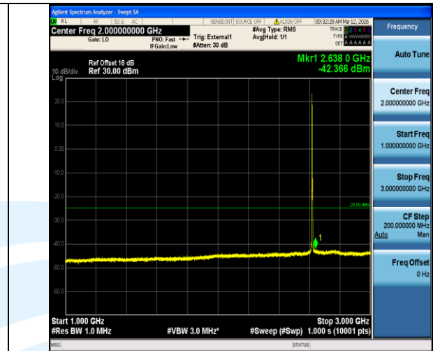
Band38-5MHz-QPSK-38225-1RB#0-1000~3000-PASS
