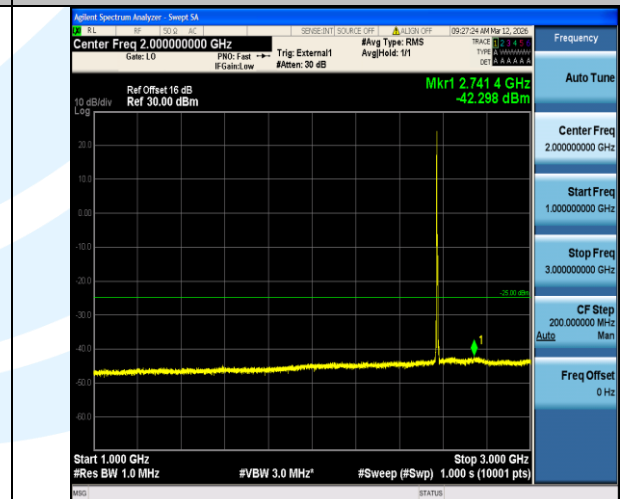
Band38-5MHz-16QAM-37775-1RB#0-1000~3000-PASS
