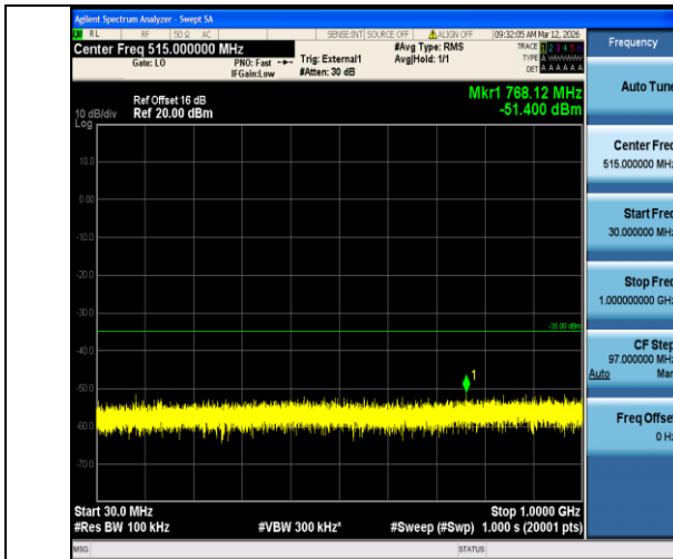
Band38-5MHz-QPSK-38225-1RB#0-30~1000-PASS
