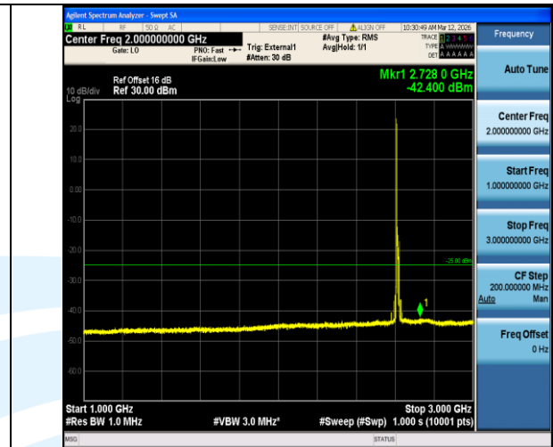
Band38-15MHz-16QAM-38175-1RB#0-1000~3000-PASS
