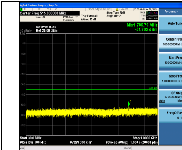
Band38-15MHz-QPSK-38175-1RB#0-30~1000-PASS
