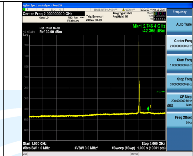
Band38-10MHz-QPSK-38200-1RB#0-1000~3000-PASS
