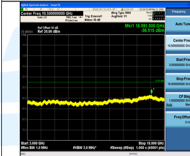
Band38-15MHz-QPSK-38175-1RB#0-3000~18000-PASS
