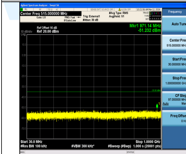
Band38-15MHz-QPSK-37825-1RB#0-30~1000-PASS
