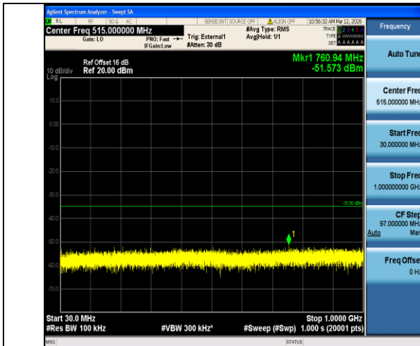
Band38-20MHz-QPSK-38150-1RB#0-30~1000-PASS
