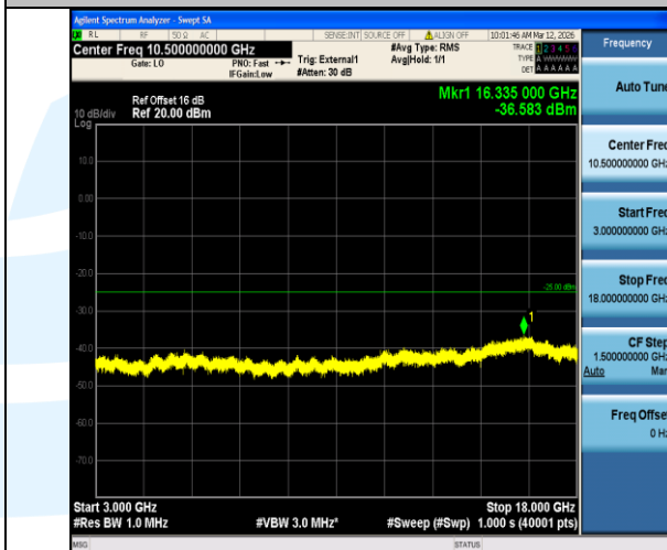
Band38-10MHz-QPSK-38200-1RB#0-3000~18000-PASS
