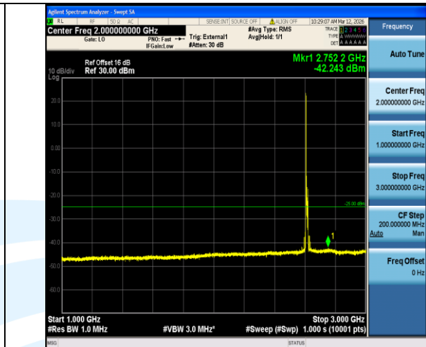
Band38-15MHz-QPSK-38175-1RB#0-1000~3000-PASS
