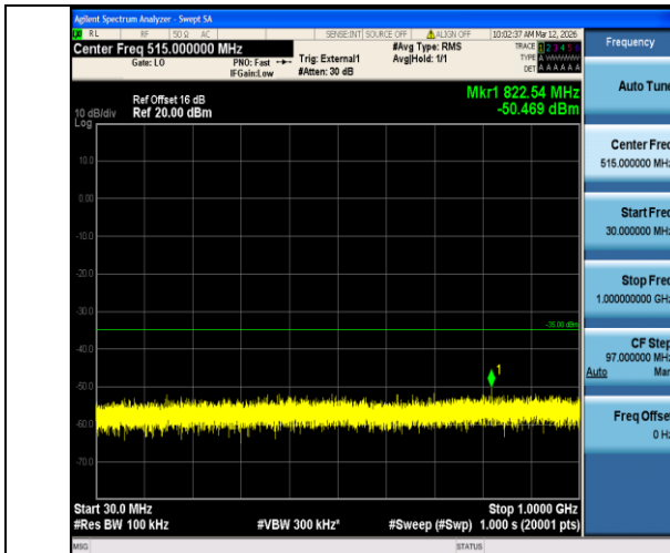
Band38-10MHz-16QAM-38200-1RB#0-30~1000-PASS
