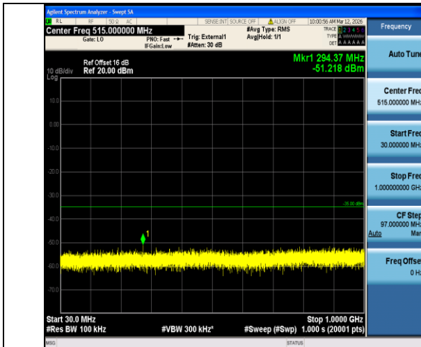
Band38-10MHz-QPSK-38200-1RB#0-30~1000-PASS
