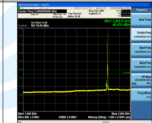
Band38-10MHz-16QAM-37800-1RB#0-1000~3000-PASS
