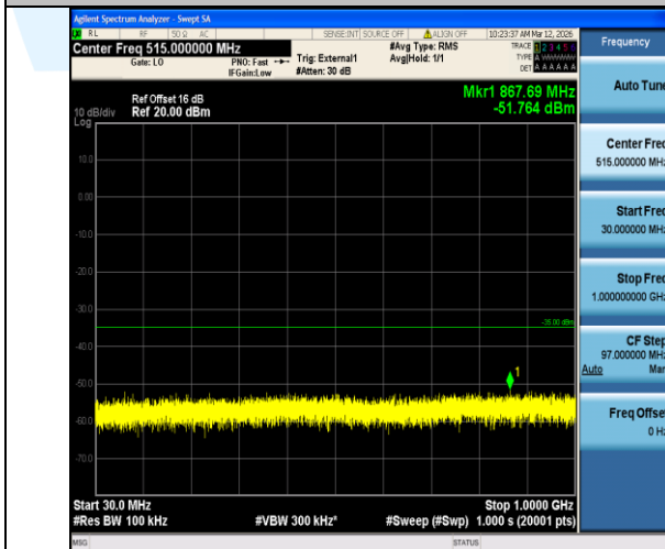
Band38-15MHz-16QAM-37825-1RB#0-30~1000-PASS
