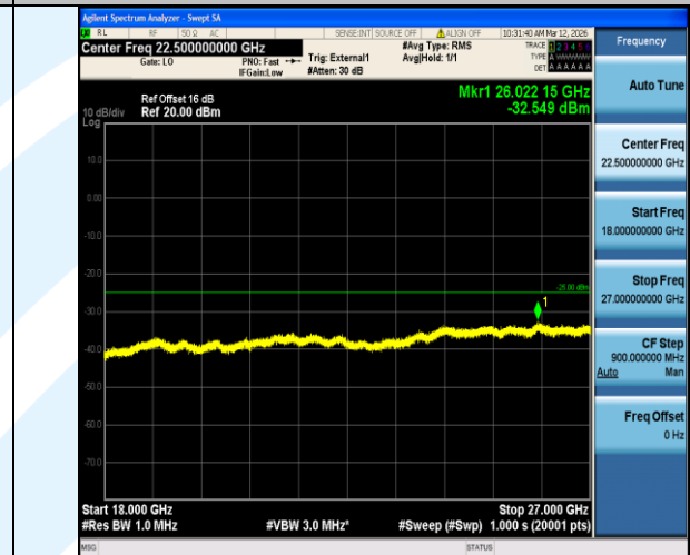
Band38-15MHz-16QAM-38175-1RB#0-18000~27000-PASS
