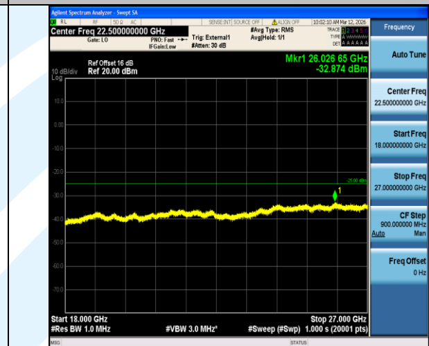
Band38-10MHz-QPSK-38200-1RB#0-18000~27000-PASS
