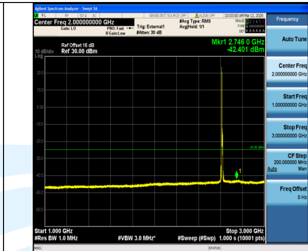
Band38-10MHz-16QAM-38200-1RB#0-1000~3000-PASS
