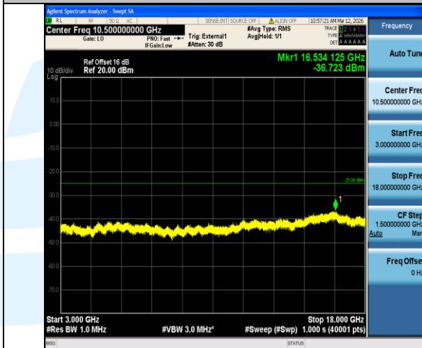
Band38-20MHz-QPSK-38150-1RB#0-3000~18000-PASS
