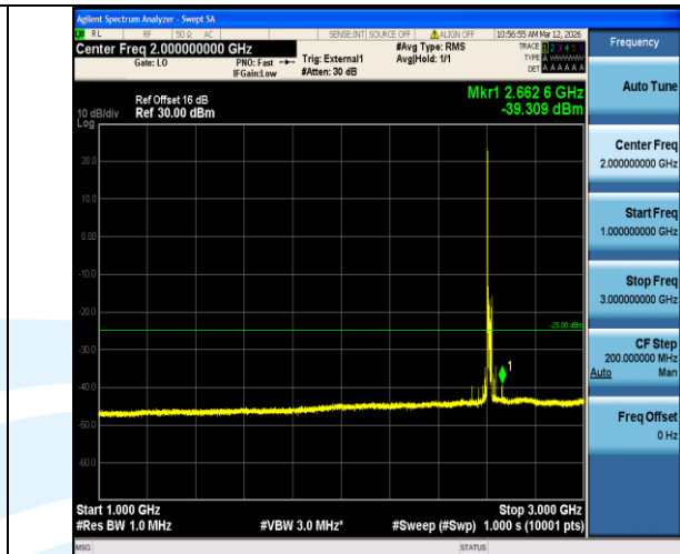
Band38-20MHz-QPSK-38150-1RB#0-1000~3000-PASS
