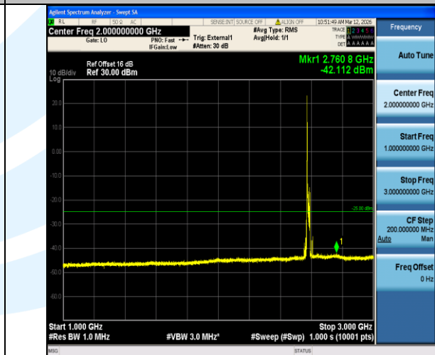
Band38-20MHz-16QAM-37850-1RB#0-1000~3000-PASS
