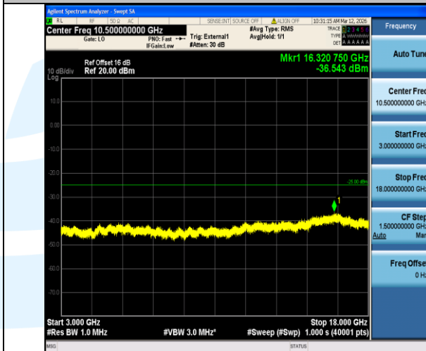
Band38-15MHz-16QAM-38175-1RB#0-3000~18000-PASS
