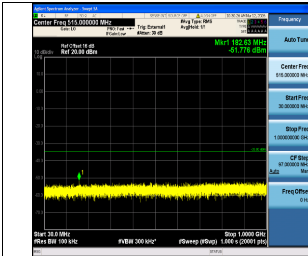
Band38-15MHz-16QAM-38175-1RB#0-30~1000-PASS
