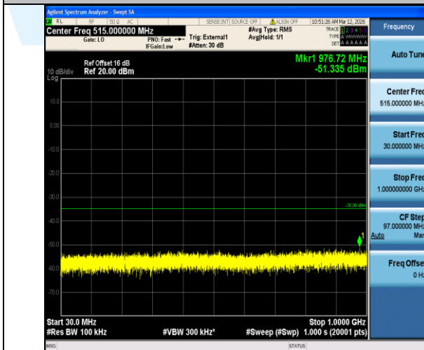
Band38-20MHz-16QAM-37850-1RB#0-30~1000-PASS
