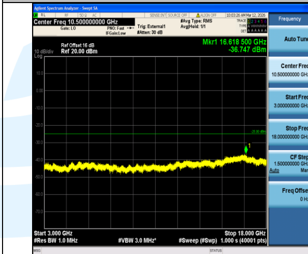
Band38-10MHz-16QAM-38200-1RB#0-3000~18000-PASS
