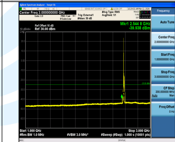
Band38-15MHz-16QAM-37825-1RB#0-1000~3000-PASS
