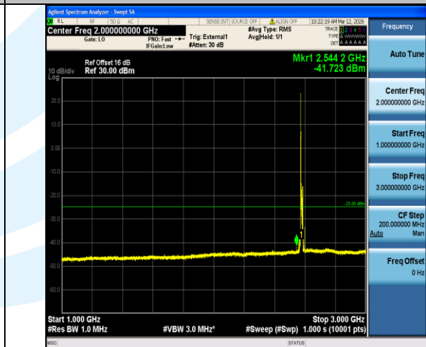
Band38-15MHz-QPSK-37825-1RB#0-1000~3000-PASS
