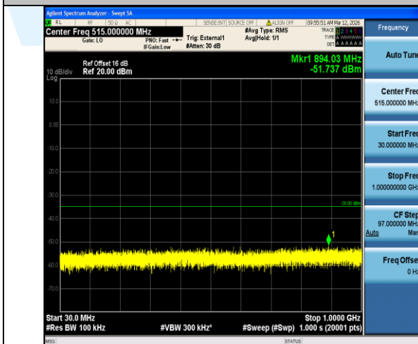
Band38-10MHz-16QAM-37800-1RB#0-30~1000-PASS
