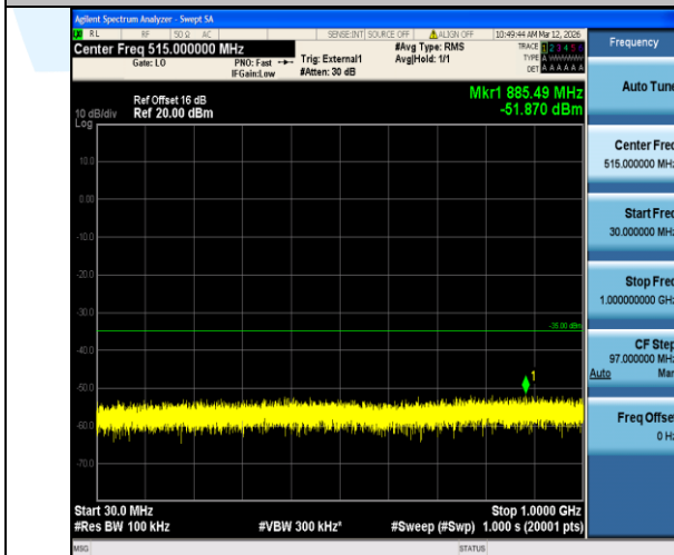
Band38-20MHz-QPSK-37850-1RB#0-30~1000-PASS
