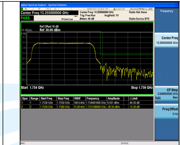
Band4-1.4MHz-QPSK-20393-6RB#0-PASS
