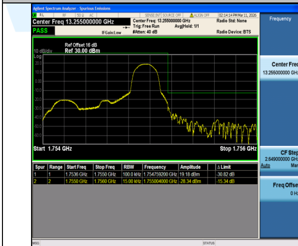
Band4-1.4MHz-16QAM-20393-1RB#5-PASS
