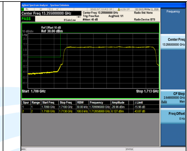
Band4-3MHz-QPSK-19965-15RB#0-PASS
