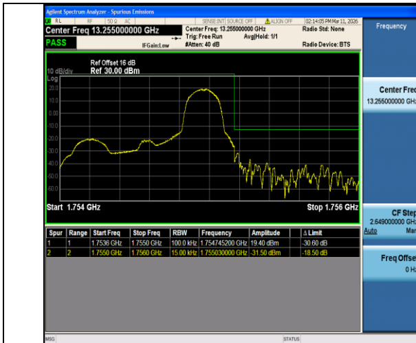
Band4-1.4MHz-QPSK-20393-1RB#5-PASS
