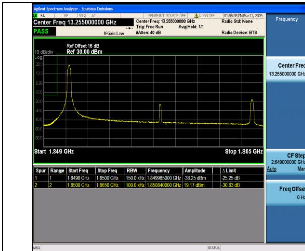
Band2-15MHz-QPSK-18675-1RB#0-PASS
