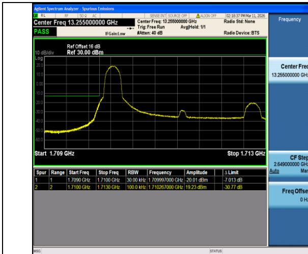
Band4-3MHz-QPSK-19965-1RB#0-PASS
