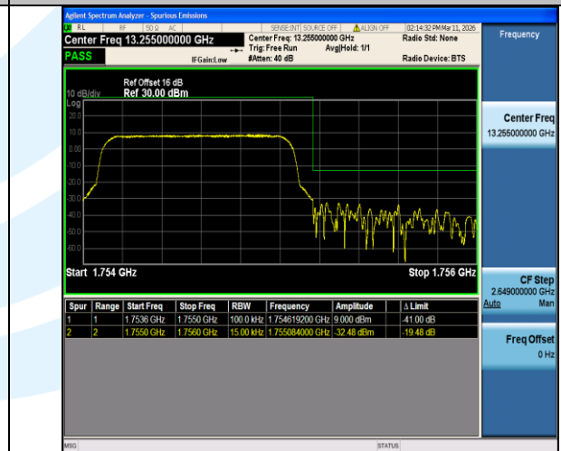
Band4-1.4MHz-16QAM-20393-6RB#0-PASS
