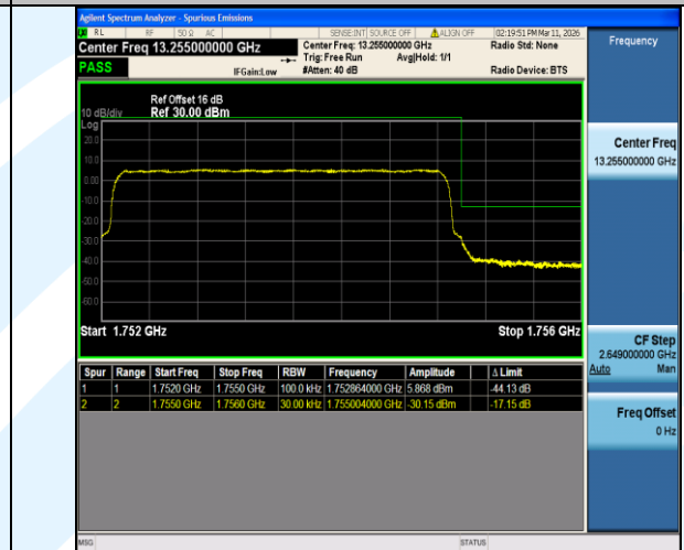
Band4-3MHz-QPSK-20385-15RB#0-PASS
