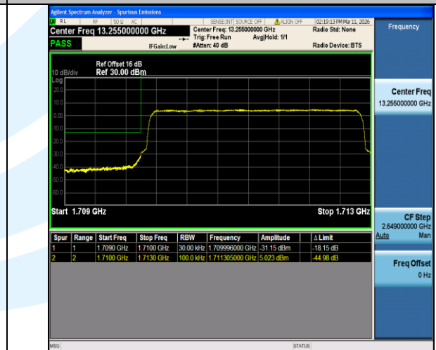
Band4-3MHz-16QAM-19965-15RB#0-PASS
