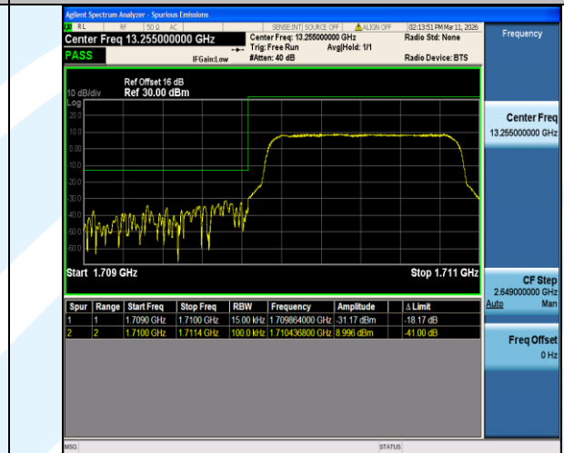
Band4-1.4MHz-16QAM-19957-6RB#0-PASS
