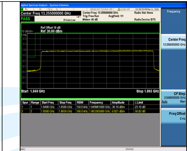
Band2-15MHz-QPSK-18675-75RB#0-PASS
