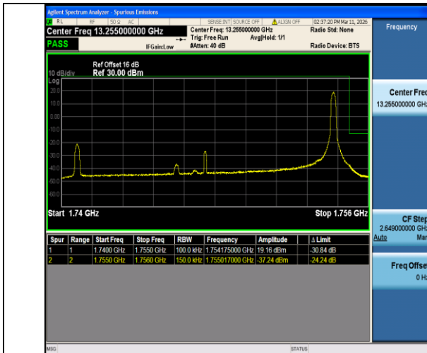
Band4-15MHz-16QAM-20325-1RB#74-PASS
