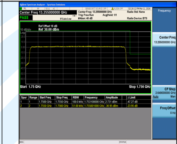
Band4-5MHz-16QAM-20375-25RB#0-PASS
