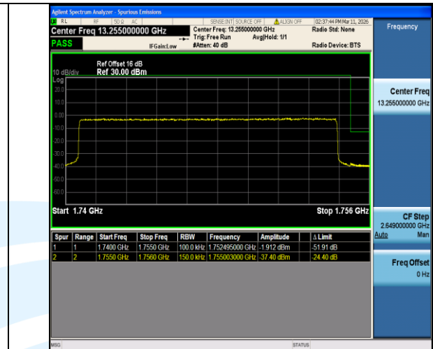
Band4-15MHz-16QAM-20325-75RB#0-PASS
