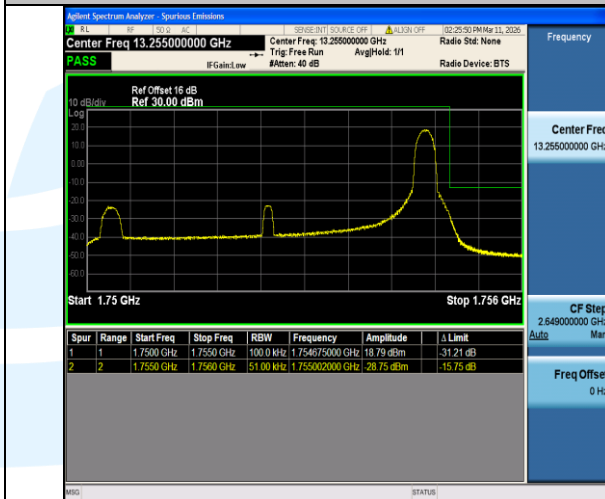
Band4-5MHz-16QAM-20375-1RB#24-PASS
