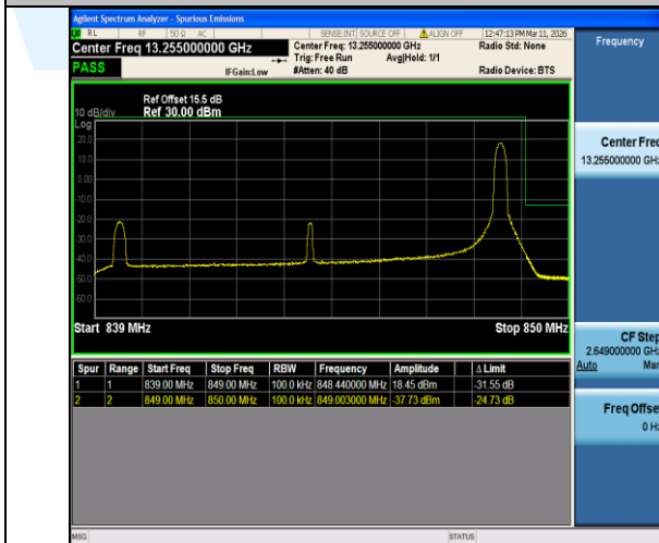
Band5-10MHz-16QAM-20600-1RB#49-PASS
