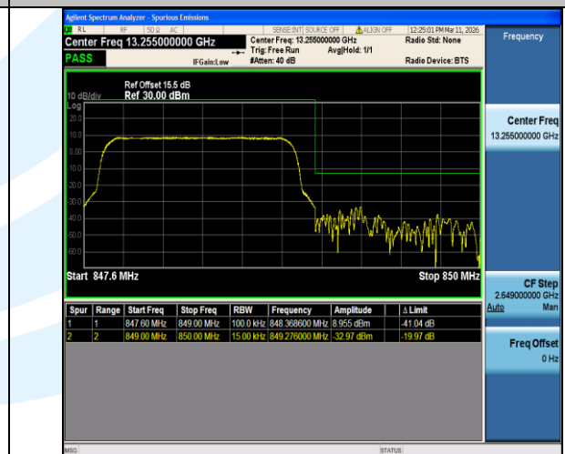
Band5-1.4MHz-16QAM-20643-6RB#0-PASS
