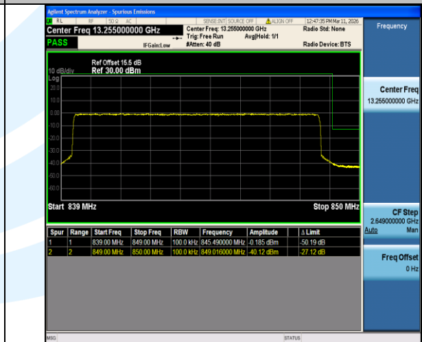
Band5-10MHz-16QAM-20600-50RB#0-PASS
