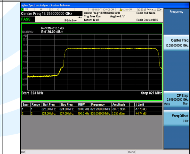
Band5-3MHz-16QAM-20415-15RB#0-PASS
