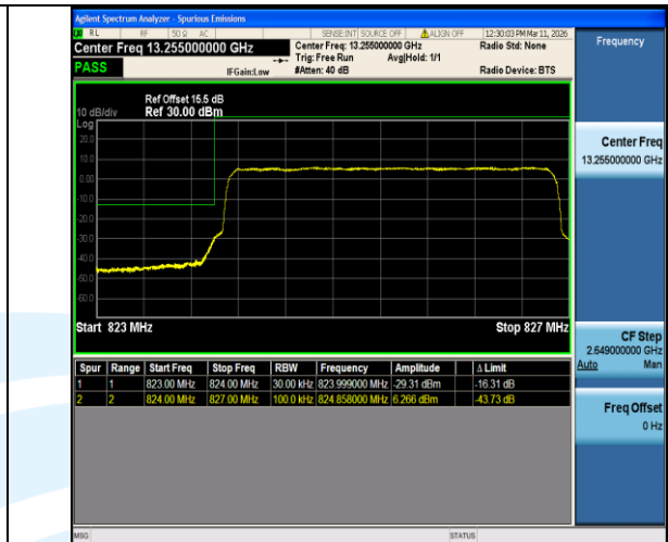
Band5-3MHz-QPSK-20415-15RB#0-PASS
