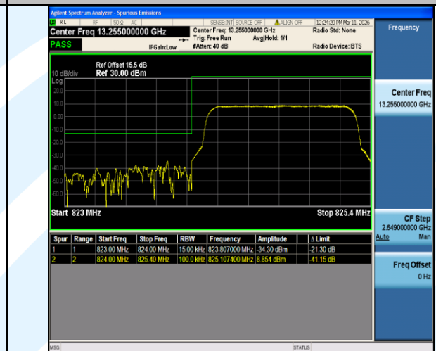
Band5-1.4MHz-16QAM-20407-6RB#0-PASS
