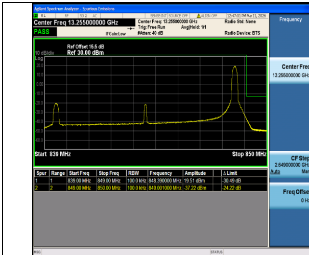
Band5-10MHz-QPSK-20600-1RB#49-PASS
