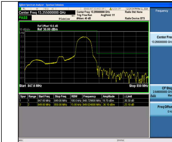
Band5-1.4MHz-QPSK-20643-1RB#5-PASS
