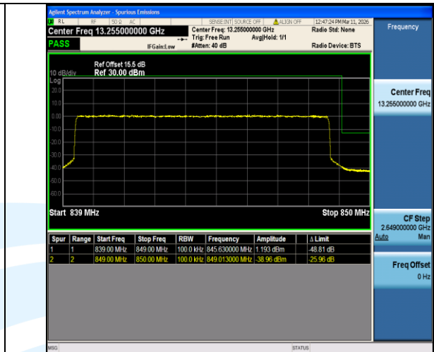
Band5-10MHz-QPSK-20600-50RB#0-PASS
