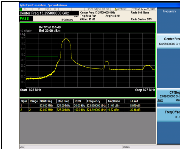
Band5-3MHz-QPSK-20415-1RB#0-PASS
