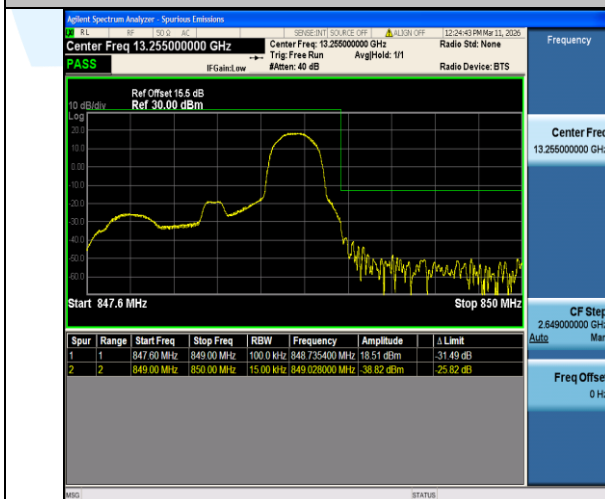
Band5-1.4MHz-16QAM-20643-1RB#5-PASS
