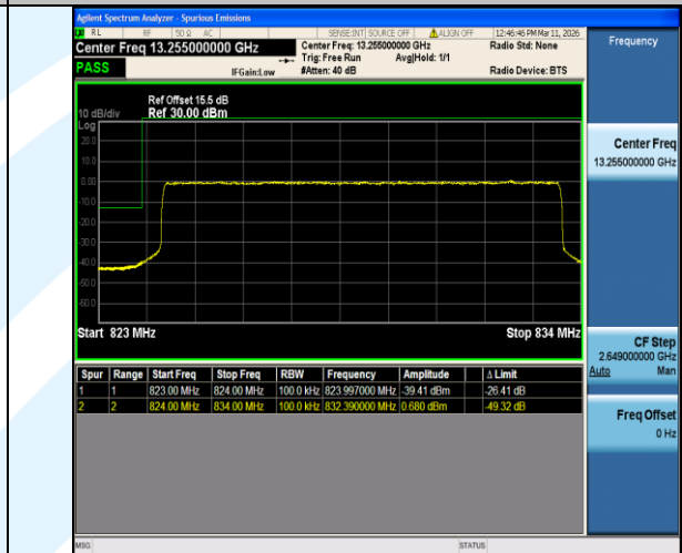
Band5-10MHz-16QAM-20450-50RB#0-PASS
