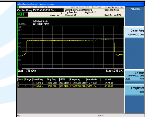
Band4-20MHz-QPSK-20300-100RB#0-PASS
