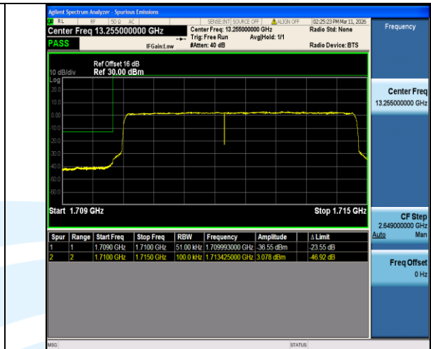
Band4-5MHz-16QAM-19975-25RB#0-PASS
