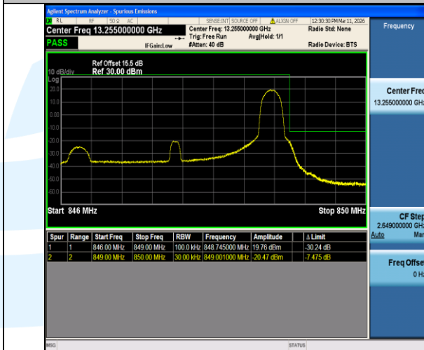
Band5-3MHz-QPSK-20635-1RB#14-PASS
