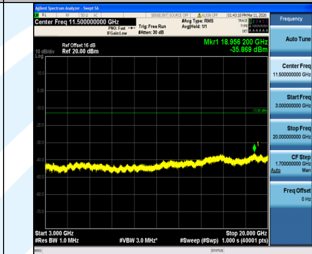
Band2-3MHz-16QAM-18615-1RB#0-3000~20000-PASS
