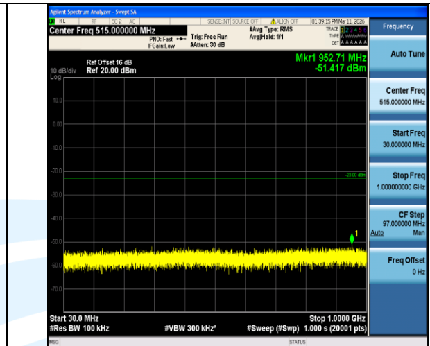
Band2-1.4MHz-16QAM-19193-1RB#0-30~1000-PASS
