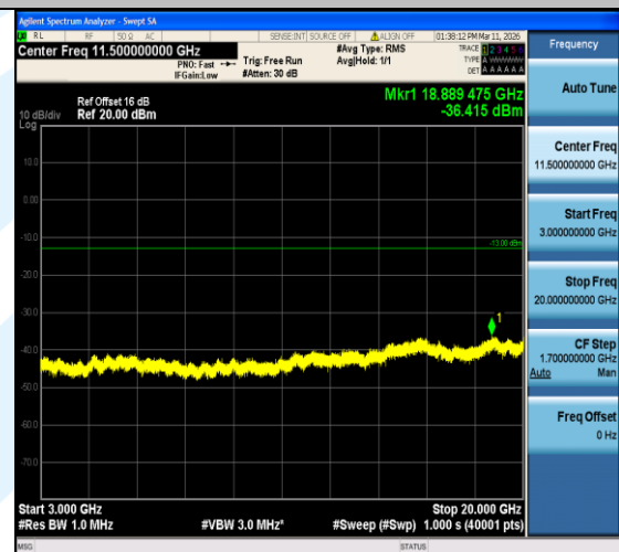
Band2-1.4MHz-QPSK-18900-1RB#0-3000~20000-PASS
