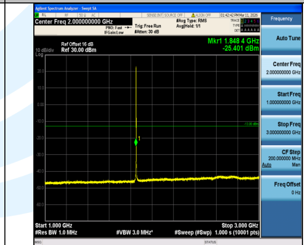
Band2-3MHz-QPSK-18615-1RB#0-1000~3000-PASS
