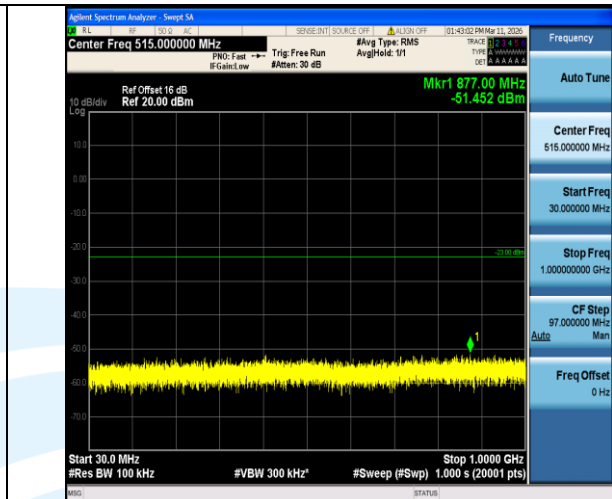
Band2-3MHz-16QAM-18615-1RB#0-30~1000-PASS
