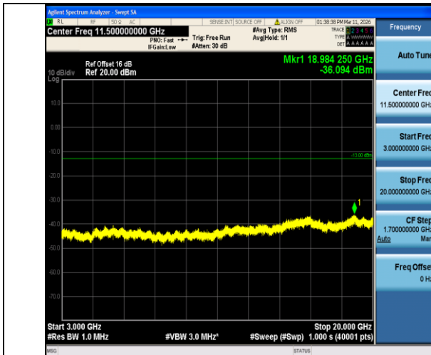
Band2-1.4MHz-16QAM-18900-1RB#0-3000~20000-PASS
