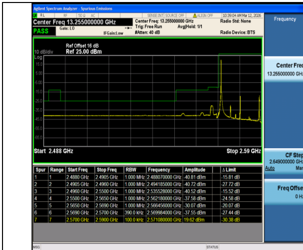
Band38-20MHz-16QAM-37850-1RB#0-PASS
