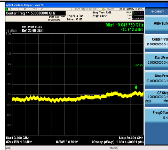
Band2-1.4MHz-QPSK-18607-1RB#0-3000~20000-PASS
