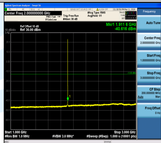
Band2-1.4MHz-QPSK-19193-1RB#0-1000~3000-PASS
