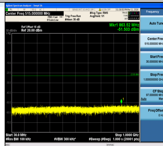
Band2-1.4MHz-QPSK-19193-1RB#0-30~1000-PASS
