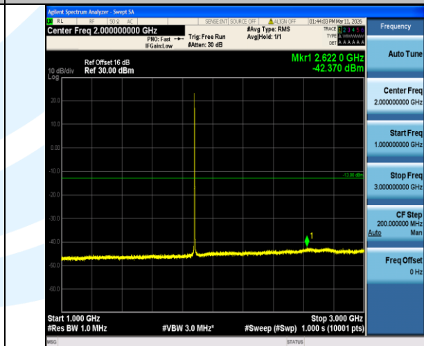
Band2-3MHz-16QAM-18900-1RB#0-1000~3000-PASS
