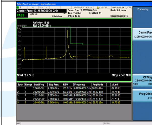
Band38-20MHz-16QAM-38150-1RB#99-PASS
