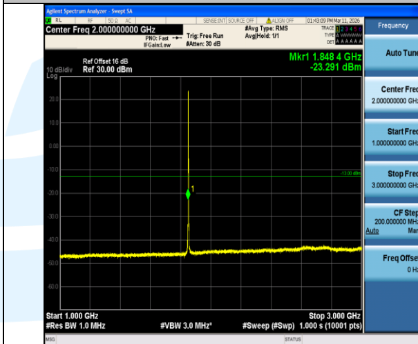
Band2-3MHz-16QAM-18615-1RB#0-1000~3000-PASS
