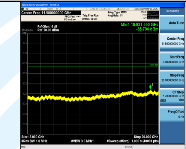
Band2-1.4MHz-16QAM-19193-1RB#0-3000~20000-PASS
