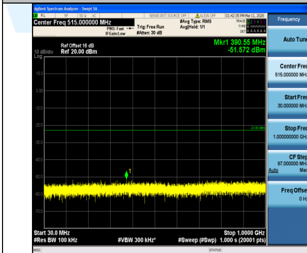
Band2-3MHz-QPSK-18615-1RB#0-30~1000-PASS
