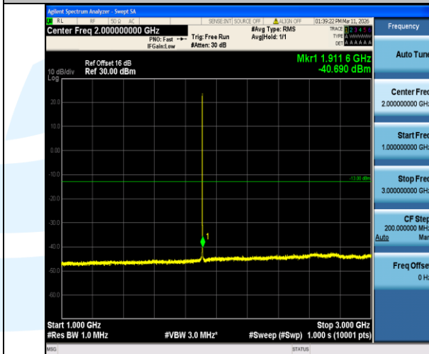
Band2-1.4MHz-16QAM-19193-1RB#0-1000~3000-PASS
