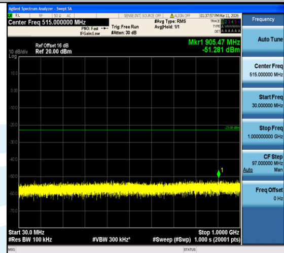
Band2-1.4MHz-QPSK-18900-1RB#0-30~1000-PASS
