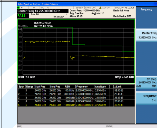
Band38-20MHz-16QAM-38150-100RB#0-PASS
