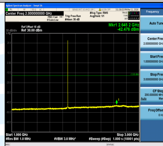
Band2-1.4MHz-QPSK-18900-1RB#0-1000~3000-PASS
