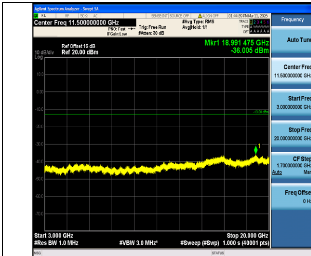
Band2-3MHz-QPSK-19185-1RB#0-3000~20000-PASS
