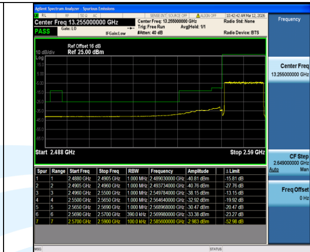
Band38-20MHz-16QAM-37850-100RB#0-PASS
