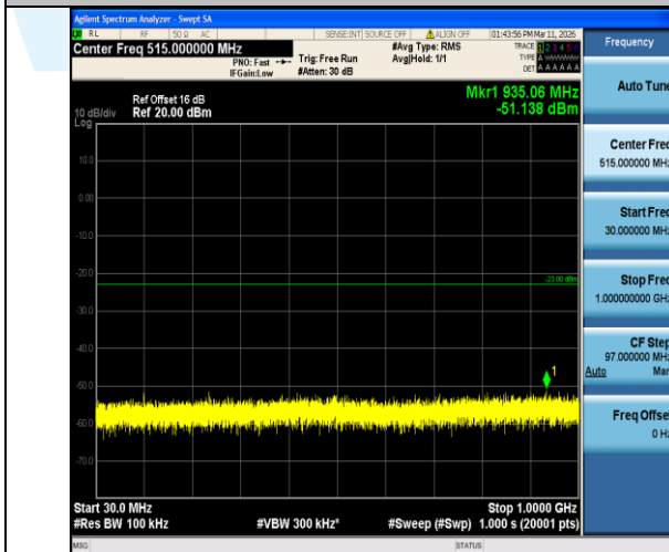
Band2-3MHz-16QAM-18900-1RB#0-30~1000-PASS
