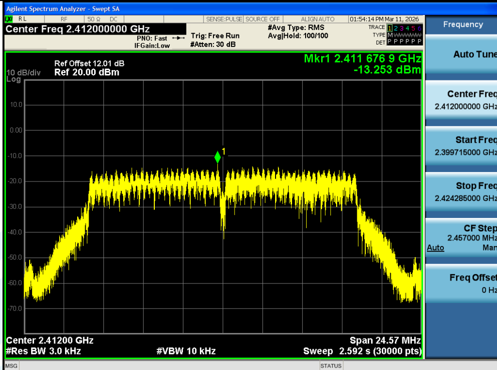
11G-Ant1-2412-PASS
