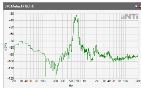
ANSI/TIA 5050-2018 \ 2N HAC OFF \ NB 12.2kbps\ 5.2 Receive path – distortion and noise\ LTE Band 13
