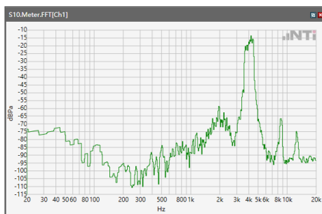
ANSI/TIA 5050-2018 \ 2N HAC OFF \ WB 12.2kbps\ 5.2 Receive path – distortion and noise\ LTE Band 7
