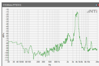
ANSI/TIA 5050-2018 \ 2N HAC OFF \ WB 12.2kbps\ 5.2 Receive path – distortion and noise\ 5GNRn66
