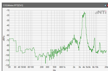
ANSI/TIA 5050-2018 \ 2N HAC OFF \ WB 12.2kbps\ 5.2 Receive path – distortion and noise\ 5GNRn77
