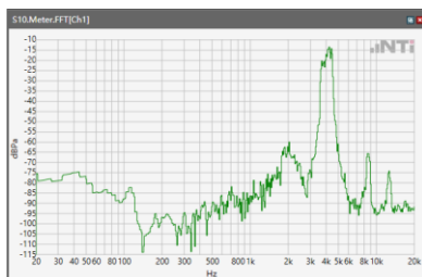
ANSI/TIA 5050-2018 \ 2N HAC OFF \ WB 12.2kbps\ 5.2 Receive path – distortion and noise\ LTE Band 12
