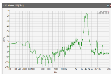
ANSI/TIA 5050-2018 \ 2N HAC OFF \ WB 12.2kbps\ 5.2 Receive path – distortion and noise\5GNRn5
