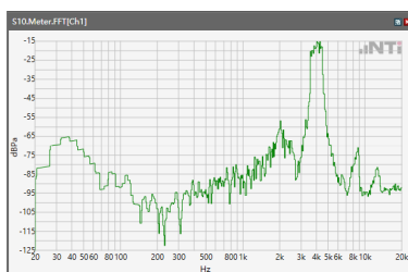
ANSI/TIA 5050-2018 \ 2N HAC OFF \ WB 12.2kbps\ 5.2 Receive path – distortion and noise\ WLAN2.4G
