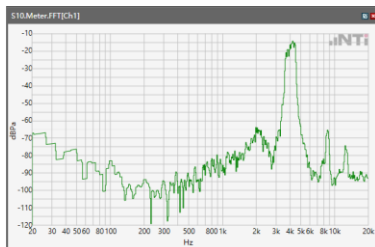
ANSI/TIA 5050-2018 \ 2N HAC OFF \ WB 12.2kbps\ 5.2 Receive path – distortion and noise\ LTE Band 66
