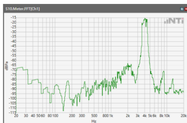
ANSI/TIA 5050-2018 \ 2N HAC OFF \ WB 12.2kbps\ 5.2 Receive path – distortion and noise\ LTE Band 13
