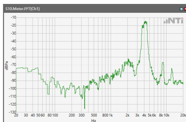
ANSI/TIA 5050-2018 \ 2N HAC OFF \ WB 12.2kbps\ 5.2 Receive path – distortion and noise\ WLAN5.2G
