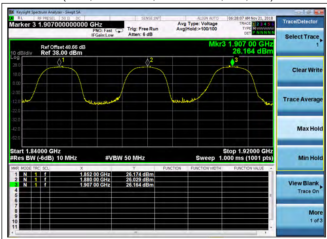
(Plot L, HSUPA Band II, Channel = 9262, 9400, 9538)
