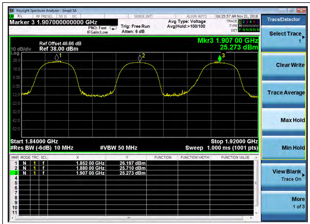
(Plot J, WCDMA Band II, Channel = 9262, 9400, 9538)
