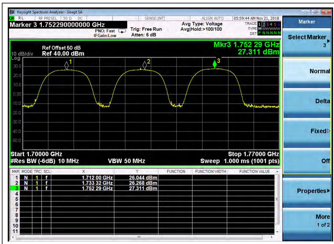
(Plot M, WCDMA Band IV, Channel = 1312, 1413, 1513)
