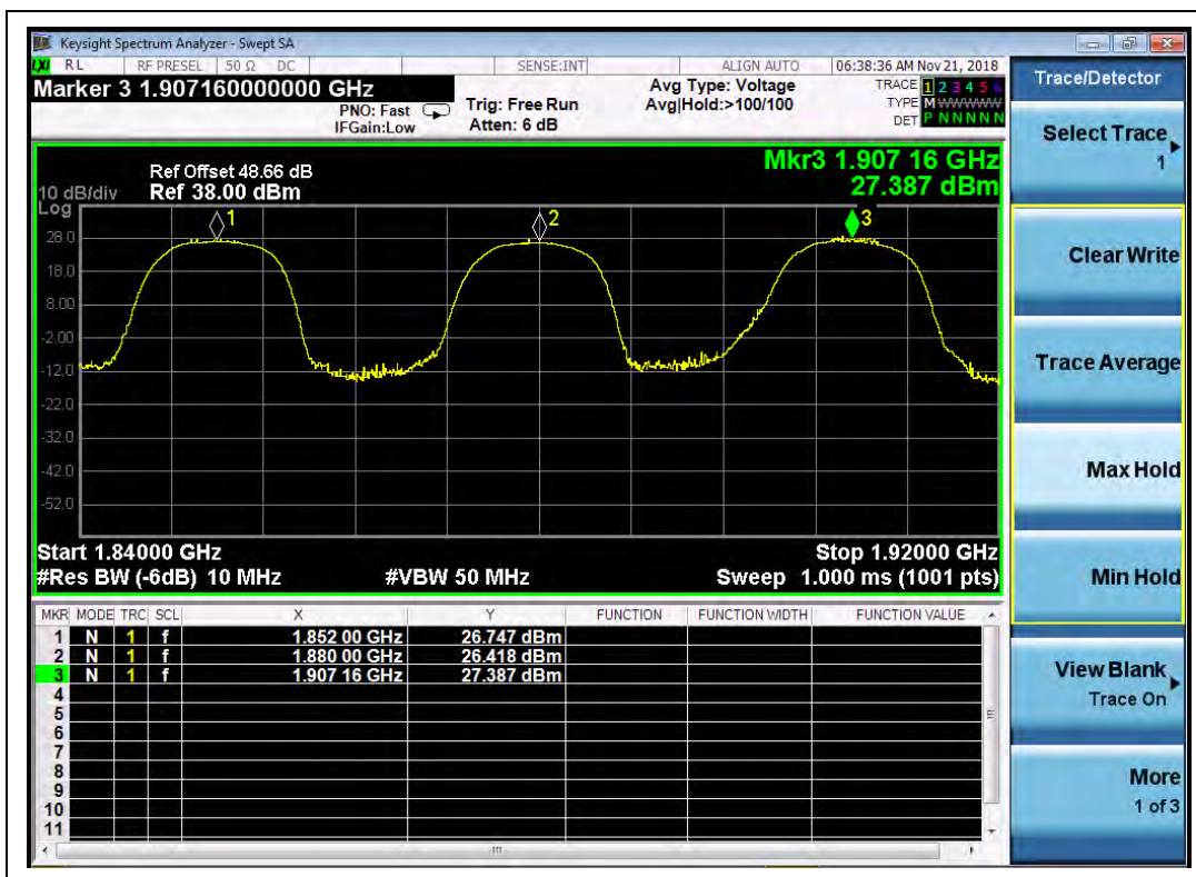
(Plot K, HSDPA Band II, Channel = 9262, 9400, 9538)
