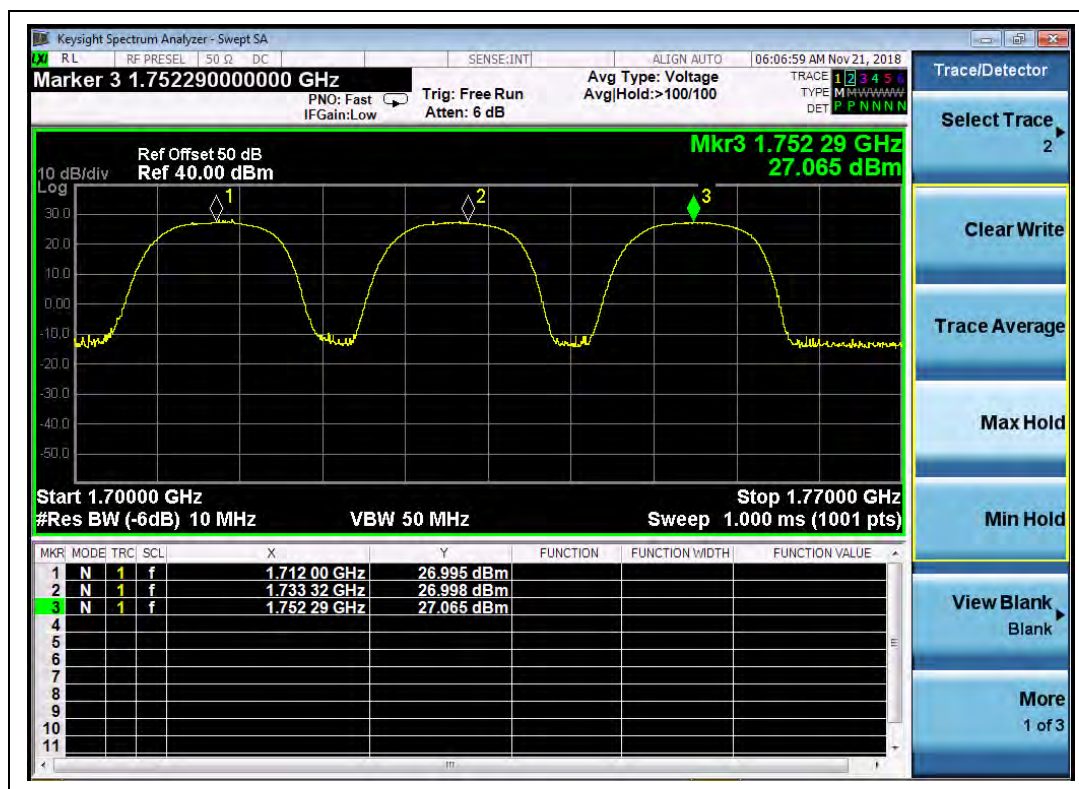
(Plot N, HSDPA Band IV, Channel = 1312, 1413, 1513)
