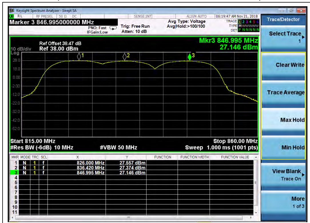
(Plot H, HSDPA Band V, Channel = 4132, 4182, 4233)
