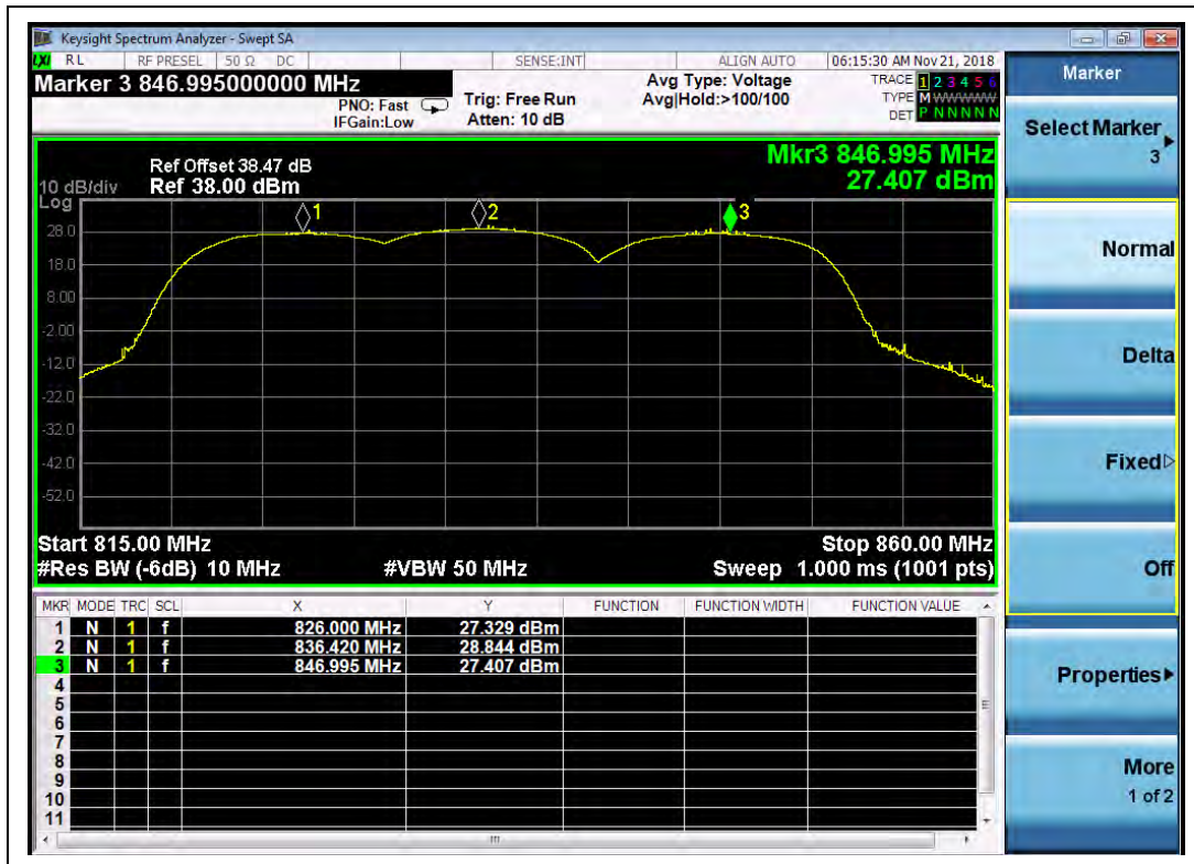
(Plot I, HSUPA Band V, Channel = 4132, 4182, 4233)
