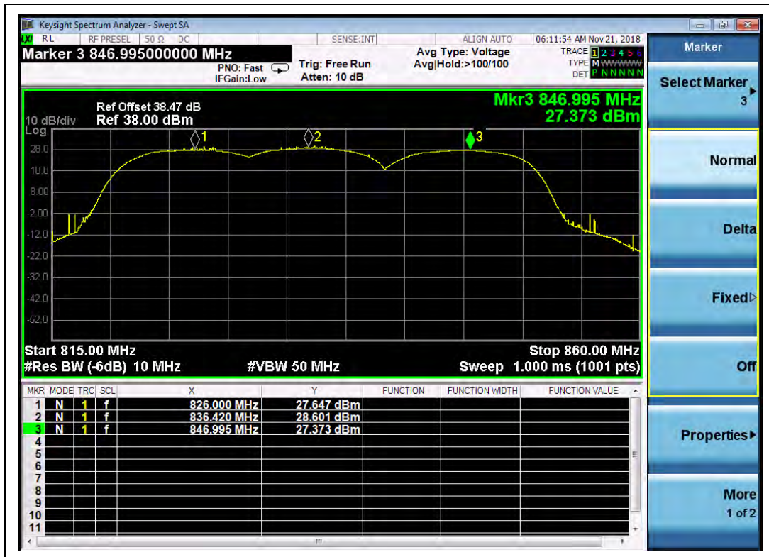
(Plot G, WCDMA Band V, Channel = 4132, 4182, 4233)
