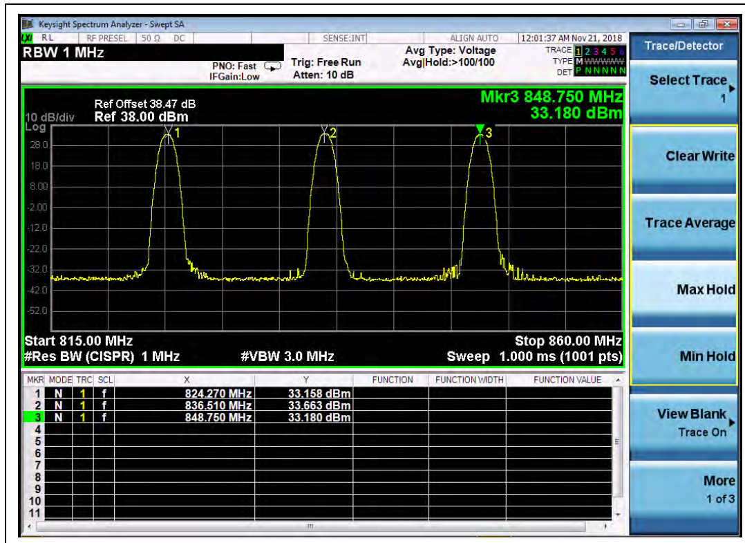
(Plot C, EDGE 850MHz, Channel = 128, 190, 251)
