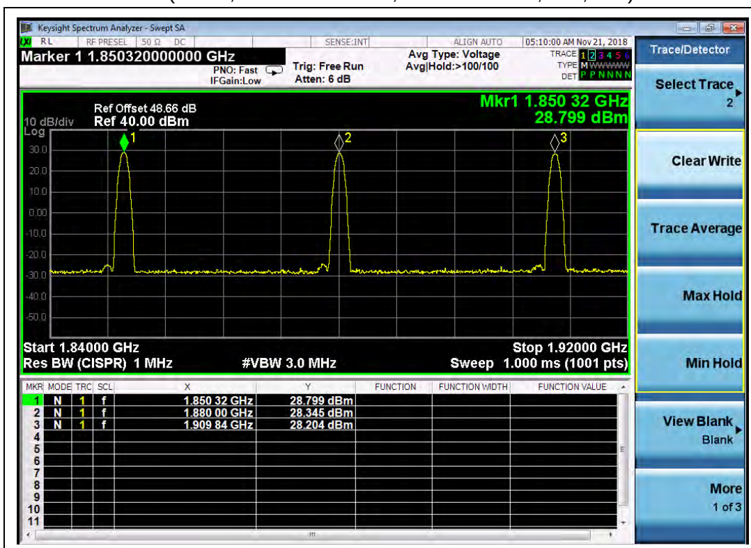
(Plot F, EDGE 1900MHz, Channel = 512, 661, 810)
