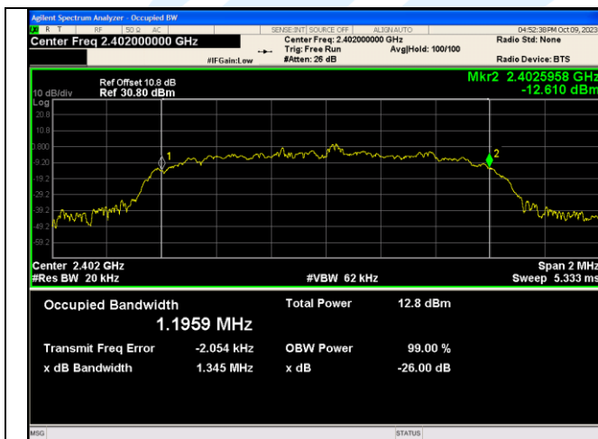
8DPSK_3-DH5_Channel 0
