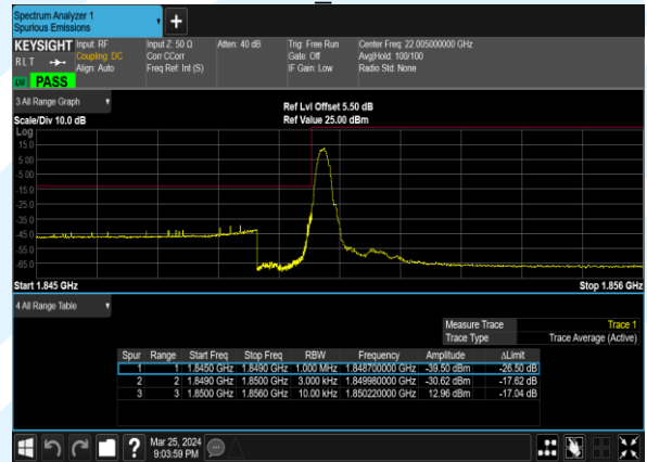
EGPRS1900 Channel512
