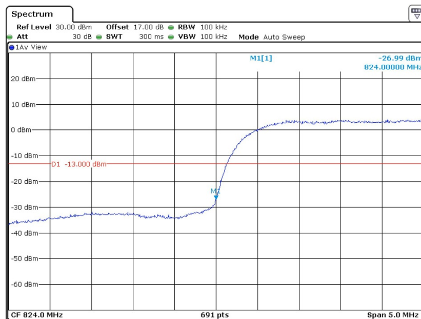
Lower Band Edge Plot on Channel 4132 (826.4 MHz)
