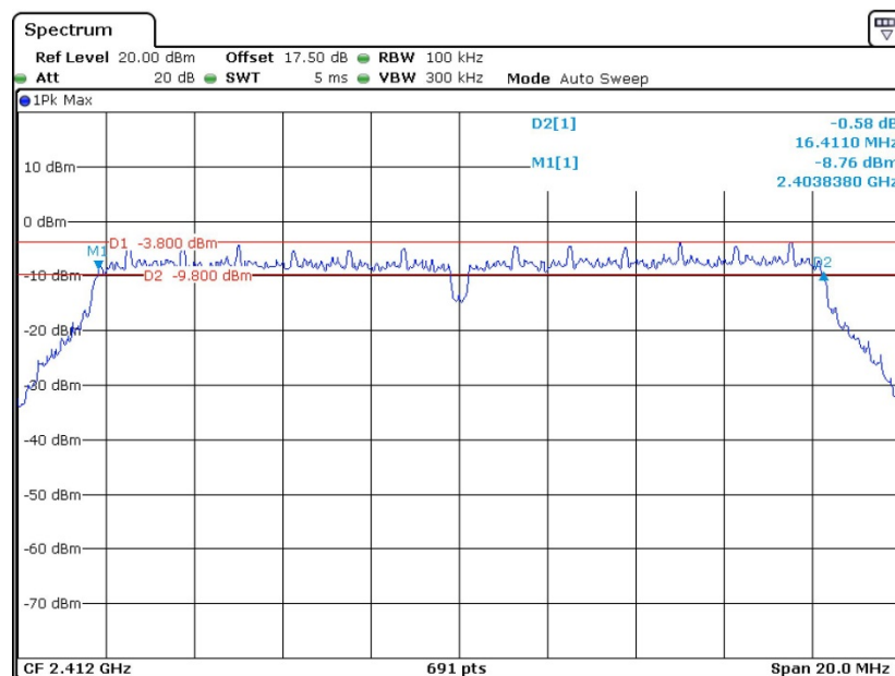
6 dB Bandwidth Plot on 802.11g Channel 01
