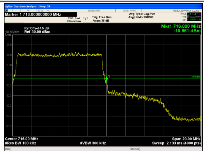
LTE Band XII - High Channel 16QAM-10
