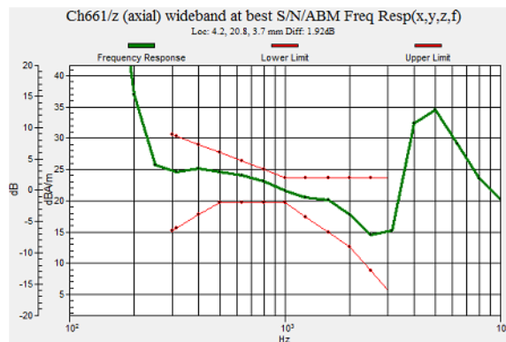
Fig 7.2 GSM1900 Ch661
