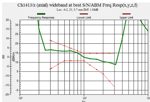
Fig 7.4 WCDMA Band IV Ch1413
