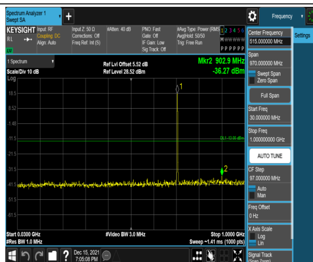
Band12-3MHz-QPSK-23165-1RB#0-Range3:30~1000MHz
