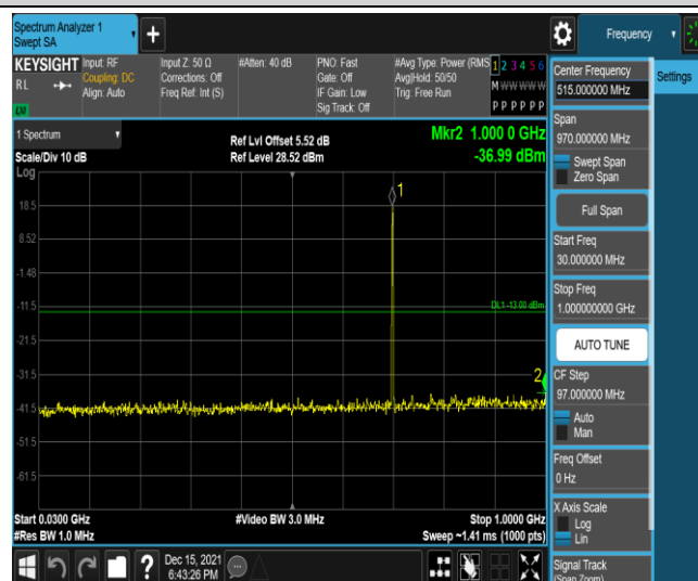
Band12-1.4MHz-QPSK-23095-1RB#0-Range3:30~1000MHz
