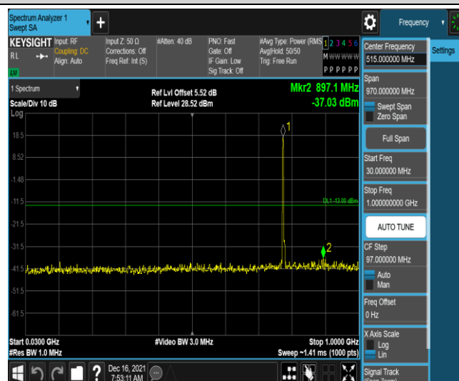
Band13-5MHz-QPSK-23230-1RB#0-Range3:30~1000MHz
