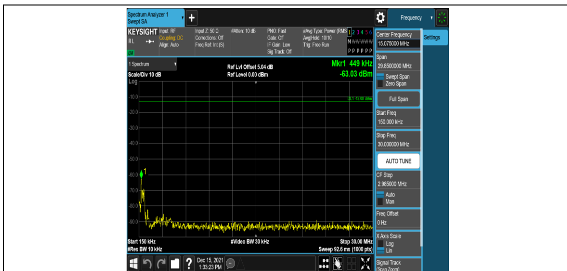
Band2-3MHz-16QAM-18615-1RB#0-Range2:0.15~30MHz
