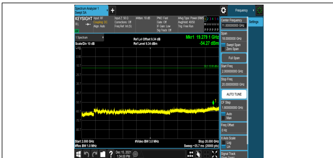
Band2-3MHz-16QAM-18615-1RB#0-Range5:2000~20000MHz
