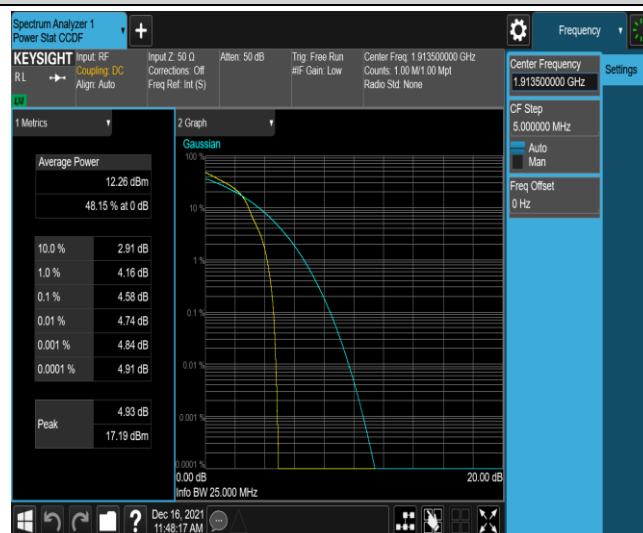
Band25-3MHz-16QAM-26675-1RB#0
