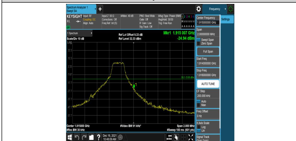
Band25-1.4MHz-16QAM-26683-1RB#5
