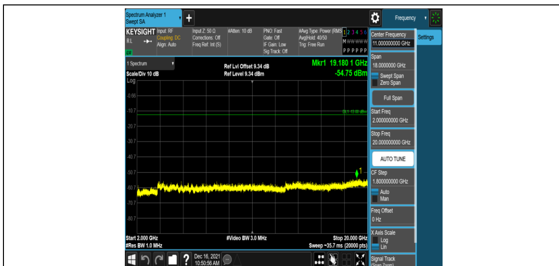
Band25-1.4MHz-16QAM-26047-1RB#0-Range5:2000~20000MHz
