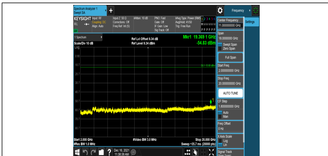
Band25-3MHz-QPSK-26055-1RB#0-Range5:2000~20000MHz
