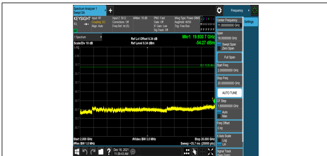
Band25-3MHz-16QAM-26055-1RB#0-Range5:2000~20000MHz
