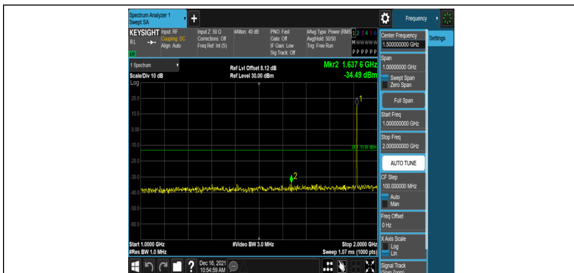
Band25-1.4MHz-16QAM-26683-1RB#0-Range4:1000~2000MHz
