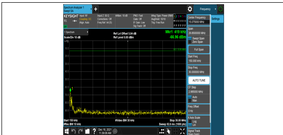
Band25-3MHz-16QAM-26055-1RB#0-Range2:0.15~30MHz
