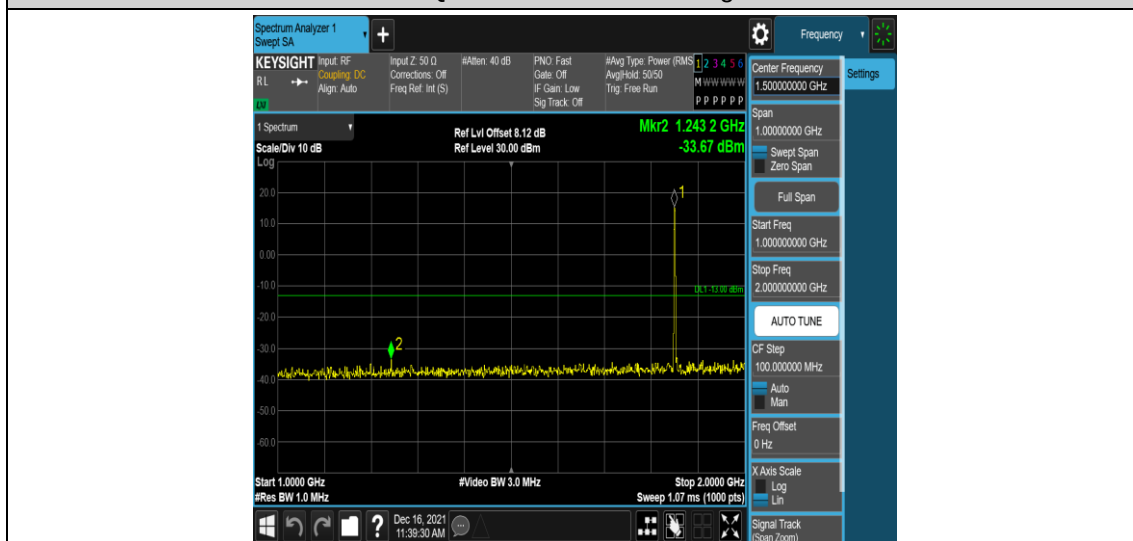
Band25-3MHz-16QAM-26055-1RB#0-Range4:1000~2000MHz
