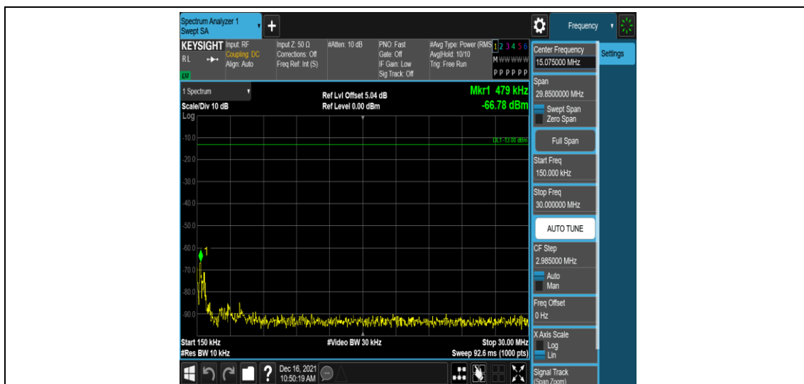
Band25-1.4MHz-16QAM-26047-1RB#0-Range2:0.15~30MHz
