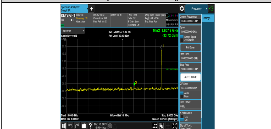
Band25-1.4MHz-16QAM-26047-1RB#0-Range4:1000~2000MHz
