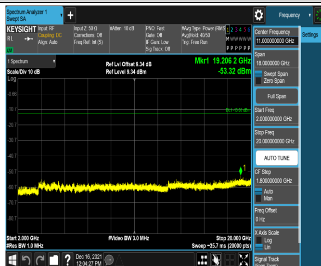
Band25-5MHz-QPSK-26665-1RB#0-Range5:2000~20000MHz
