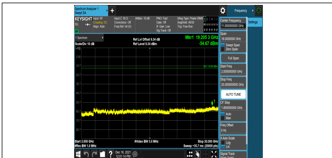
Band25-5MHz-16QAM-26065-1RB#0-Range5:2000~20000MHz
