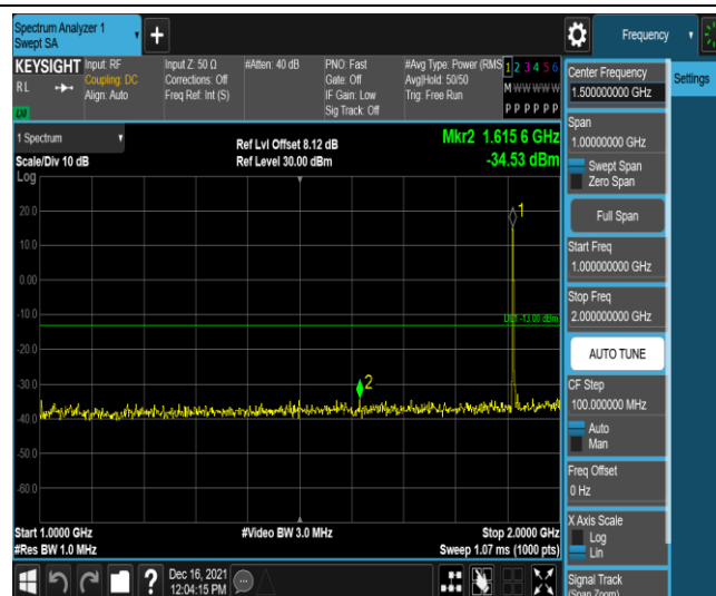
Band25-5MHz-QPSK-26665-1RB#0-Range4:1000~2000MHz
