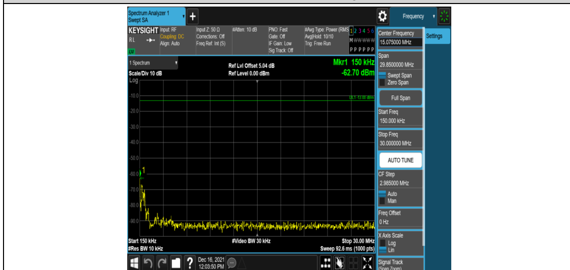
Band25-5MHz-QPSK-26665-1RB#0-Range2:0.15~30MHz
