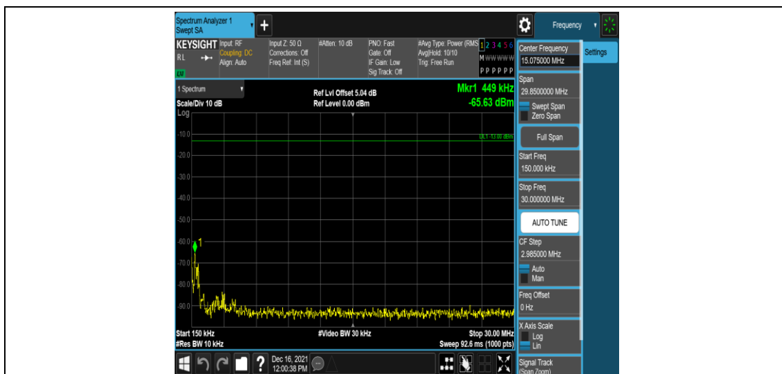
Band25-5MHz-16QAM-26065-1RB#0-Range2:0.15~30MHz
