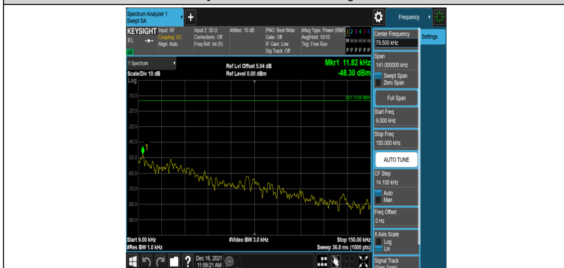
Band25-5MHz-QPSK-26065-1RB#0-Range1:0.009~0.15MHz
