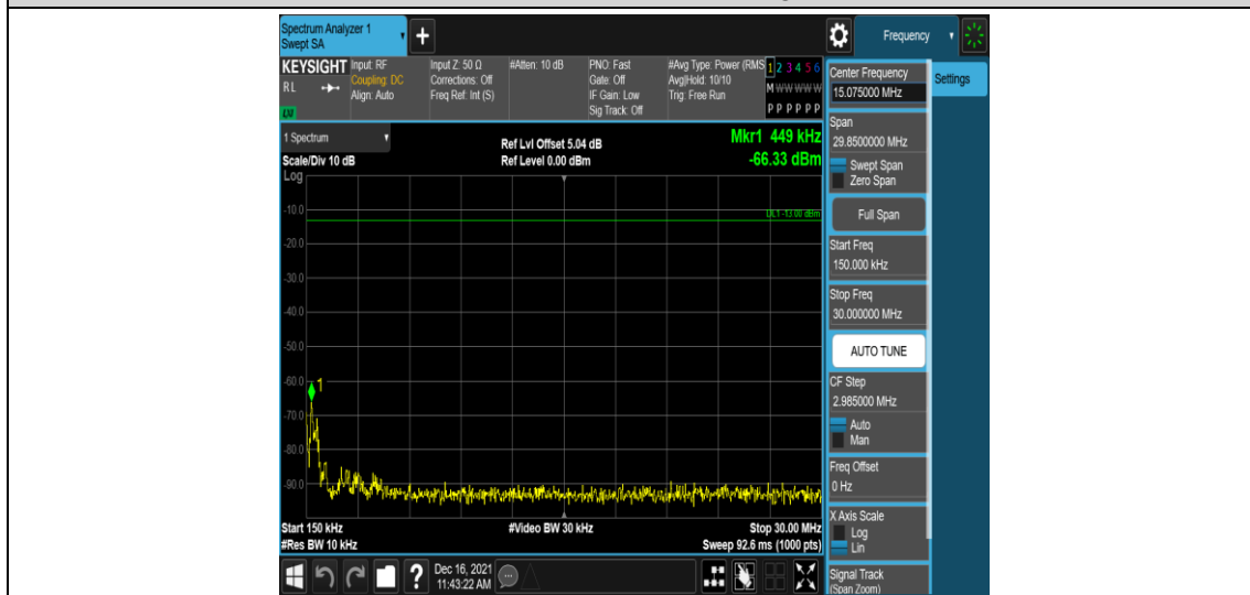
Band25-3MHz-16QAM-26675-1RB#0-Range2:0.15~30MHz
