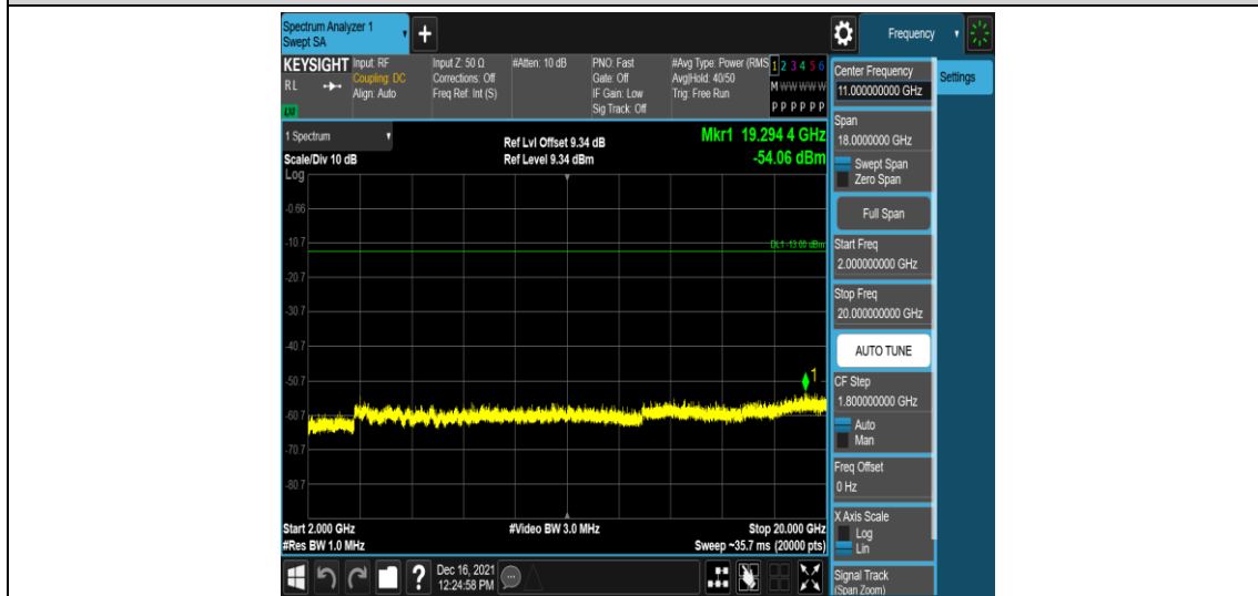
Band25-10MHz-QPSK-26640-1RB#0-Range5:2000~20000MHz
