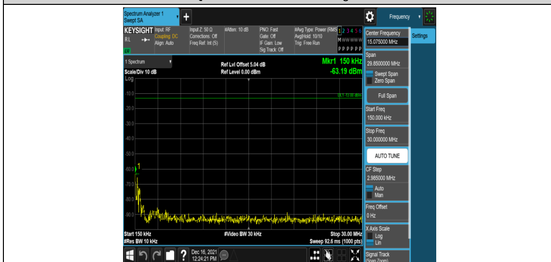
Band25-10MHz-QPSK-26640-1RB#0-Range2:0.15~30MHz
