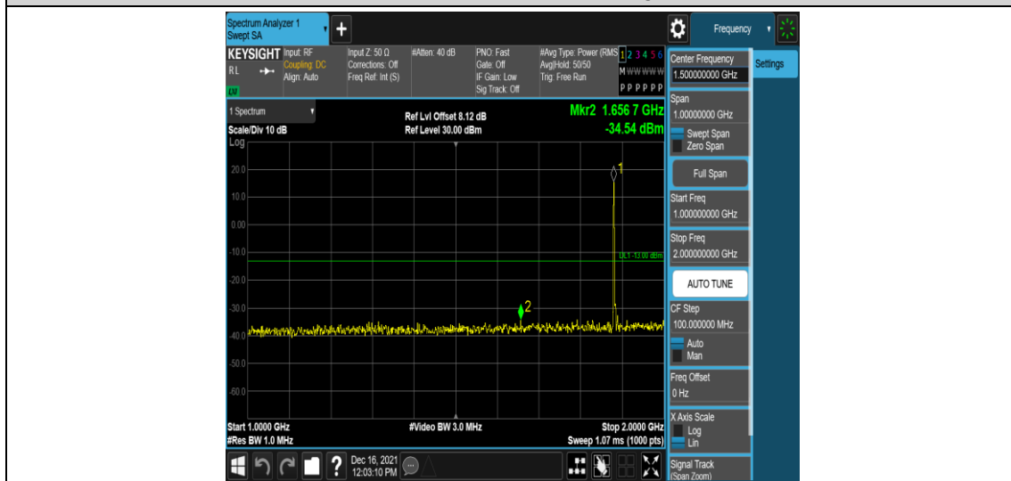
Band25-5MHz-16QAM-26365-1RB#0-Range4:1000~2000MHz
