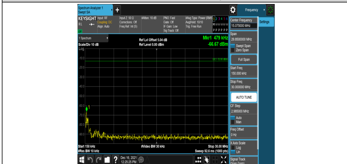
Band25-10MHz-16QAM-26640-1RB#0-Range2:0.15~30MHz
