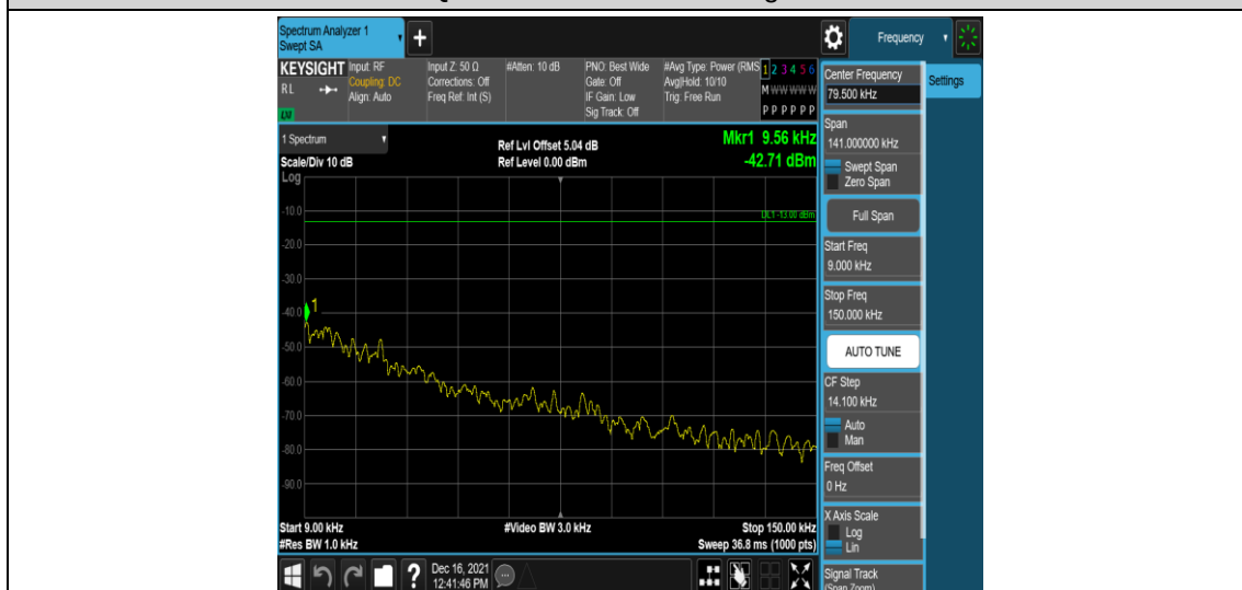
Band25-15MHz-16QAM-26115-1RB#0-Range1:0.009~0.15MHz
