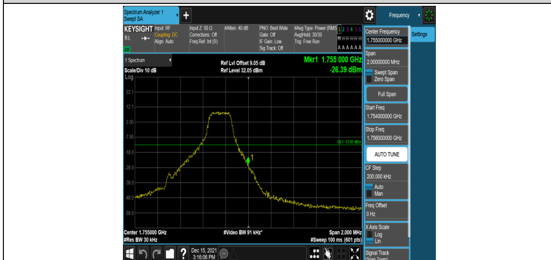
Band4-1.4MHz-16QAM-20393-1RB#5
