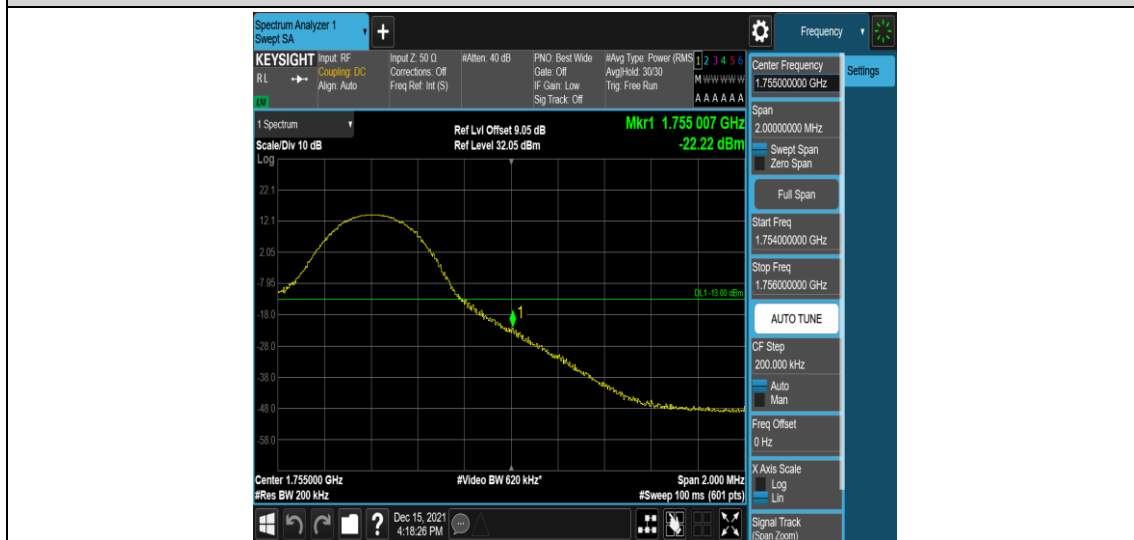
Band4-10MHz-QPSK-20350-1RB#49
