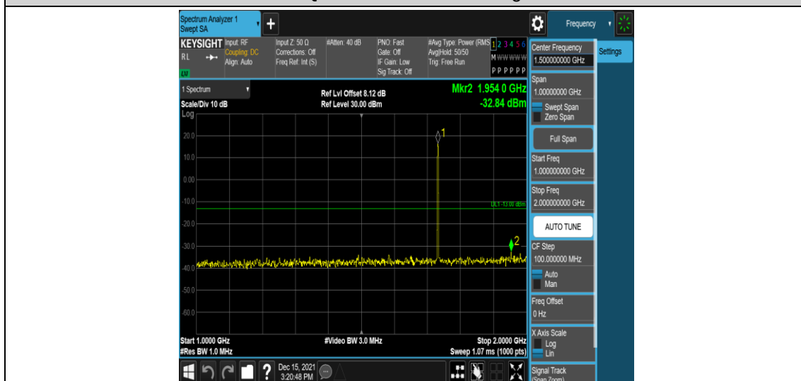
Band4-1.4MHz-16QAM-20175-1RB#0-Range4:1000~2000MHz
