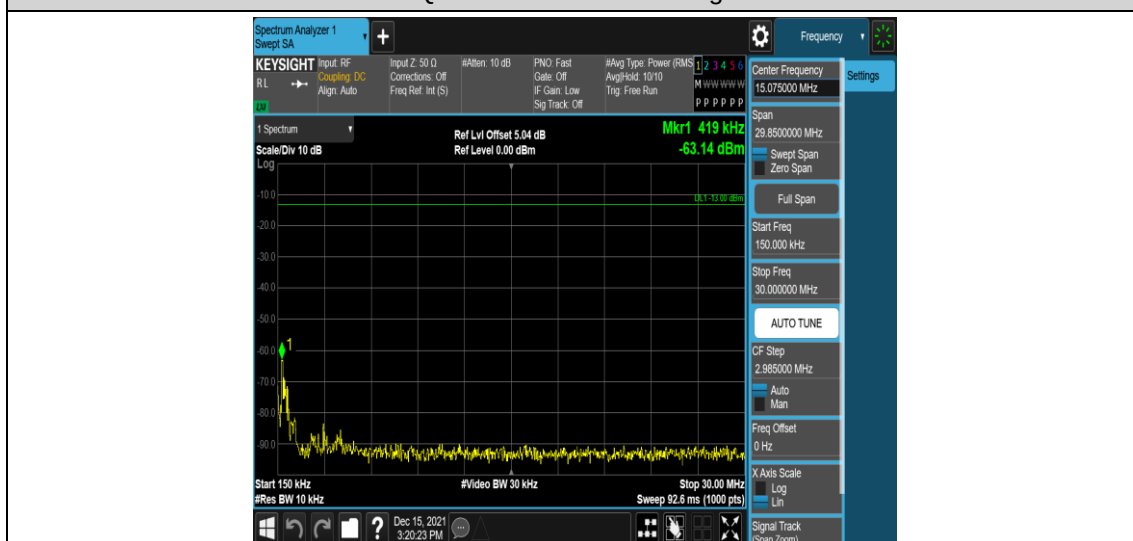
Band4-1.4MHz-16QAM-20175-1RB#0-Range2:0.15~30MHz
