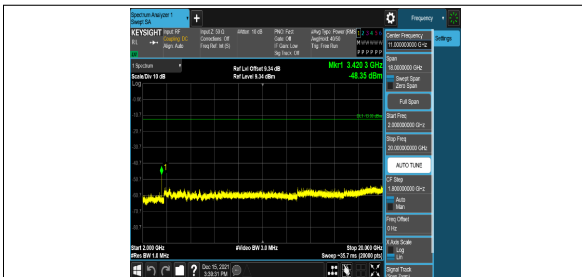
Band4-3MHz-16QAM-19965-1RB#0-Range5:2000~20000MHz
