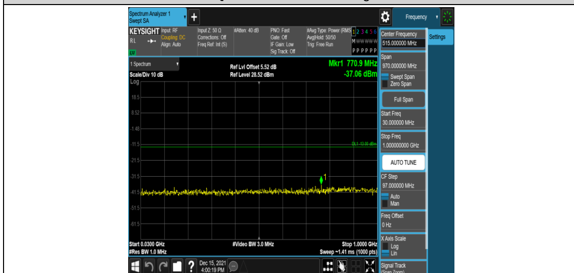
Band4-5MHz-16QAM-19975-1RB#0-Range3:30~1000MHz
