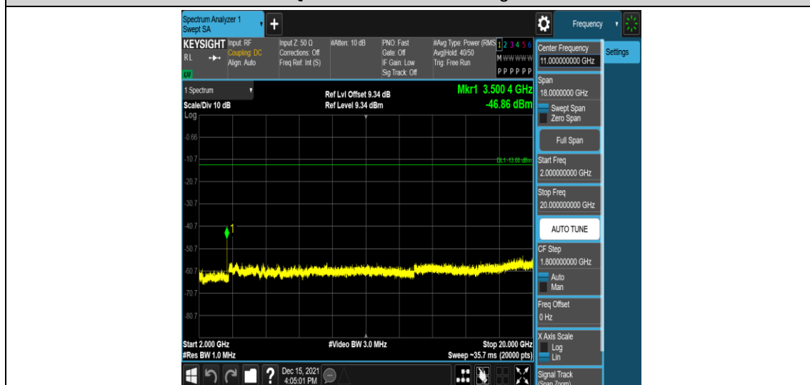
Band4-5MHz-16QAM-20375-1RB#0-Range5:2000~20000MHz
