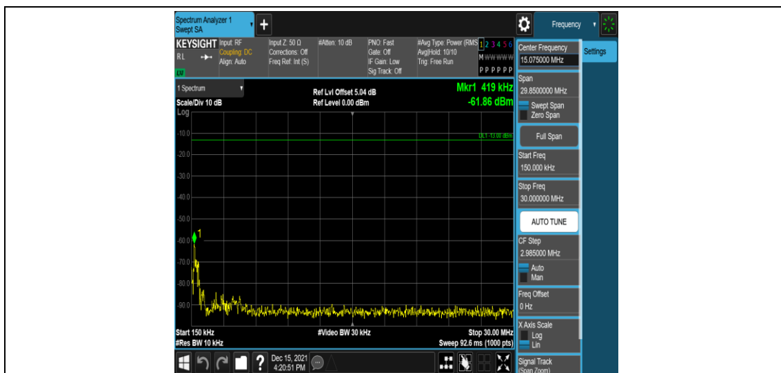
Band4-10MHz-16QAM-20000-1RB#0-Range2:0.15~30MHz
