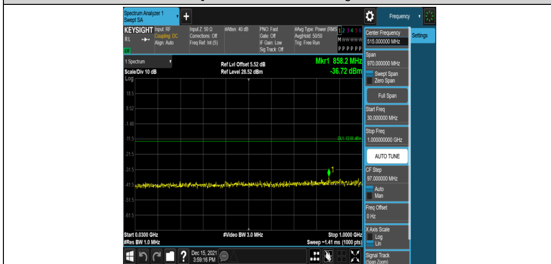
Band4-5MHz-QPSK-19975-1RB#0-Range3:30~1000MHz
