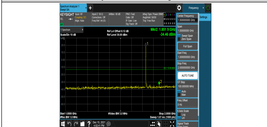
Band4-5MHz-16QAM-20175-1RB#0-Range4:1000~2000MHz
