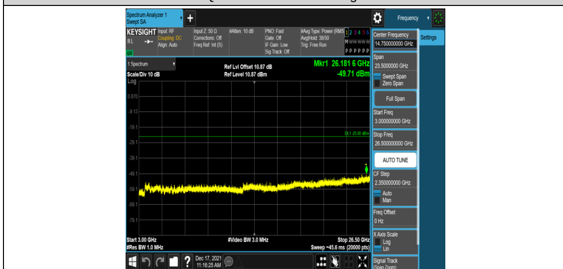
Band41-5MHz-16QAM-39675-1RB#0-Range5:3000~26500MHz
