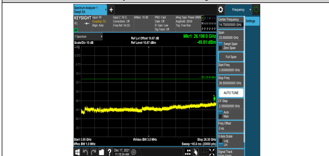
Band41-5MHz-16QAM-40620-1RB#0-Range5:3000~26500MHz
