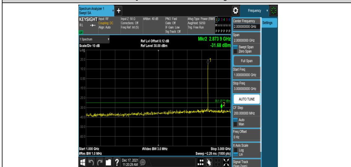
Band41-5MHz-16QAM-41565-1RB#0-Range4:1000~3000MHz
