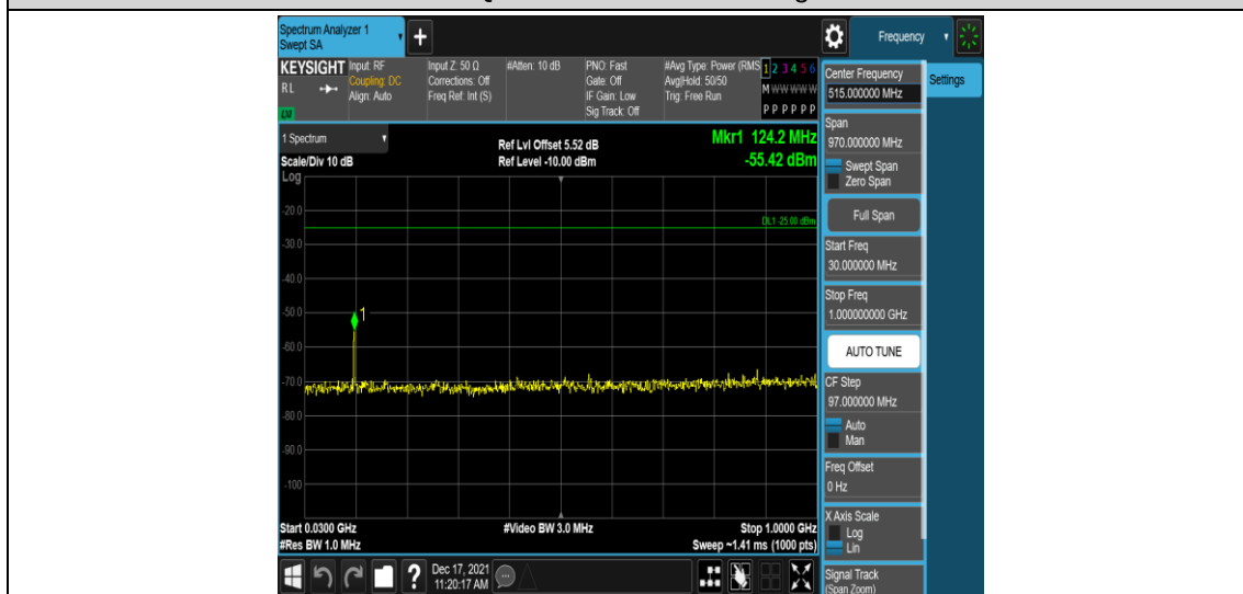
Band41-5MHz-16QAM-41565-1RB#0-Range3:30~1000MHz
