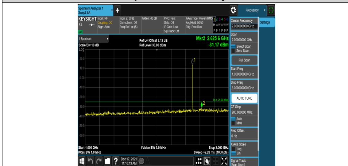
Band41-5MHz-16QAM-39675-1RB#0-Range4:1000~3000MHz
