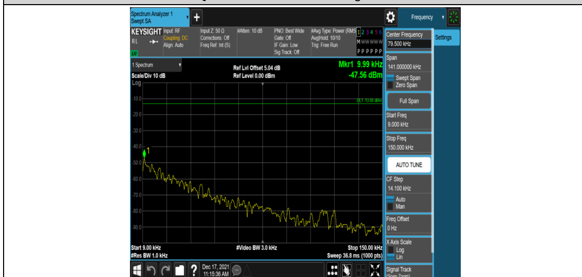
Band41-5MHz-16QAM-39675-1RB#0-Range1:0.009~0.15MHz
