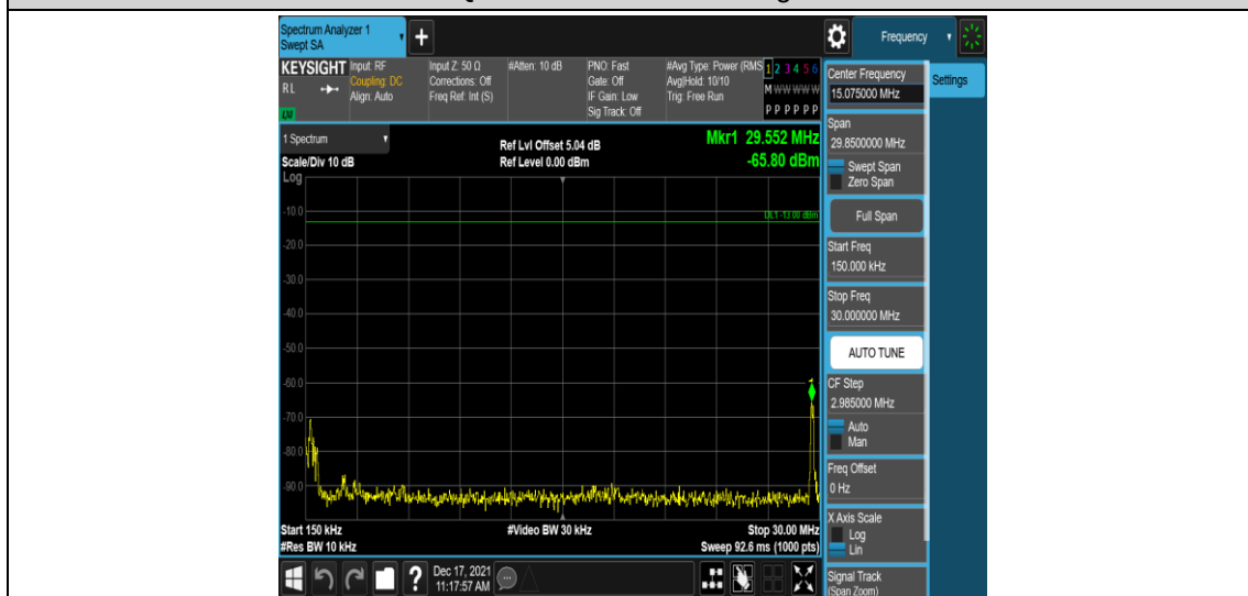
Band41-5MHz-16QAM-40620-1RB#0-Range2:0.15~30MHz
