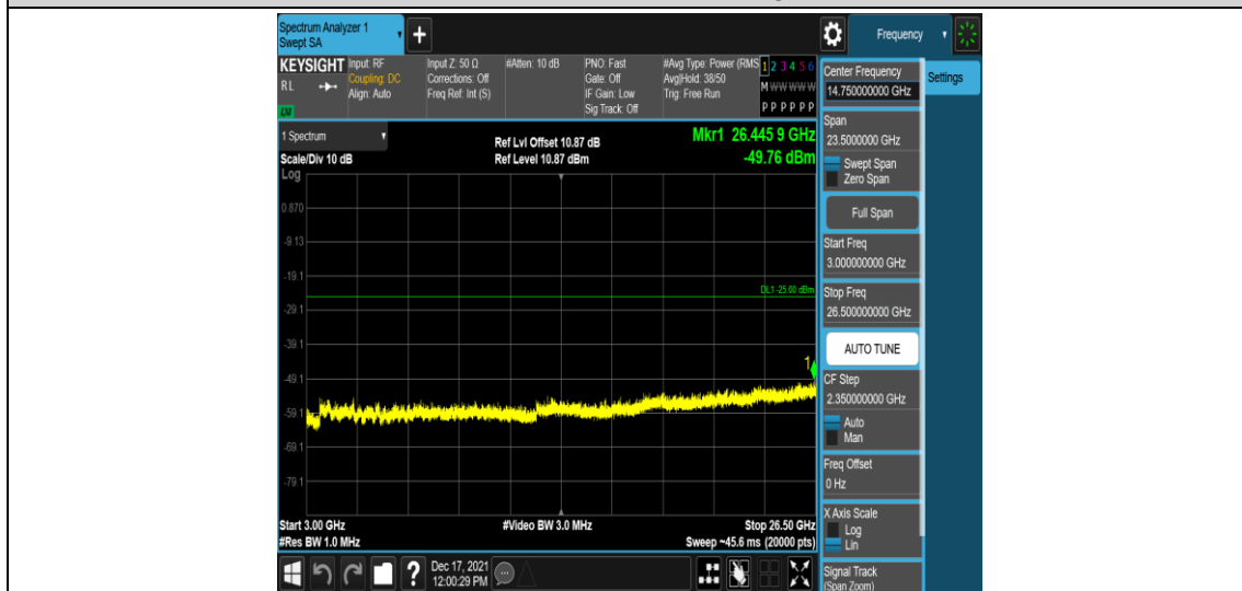
Band41-15MHz-QPSK-40620-1RB#0-Range5:3000~26500MHz
