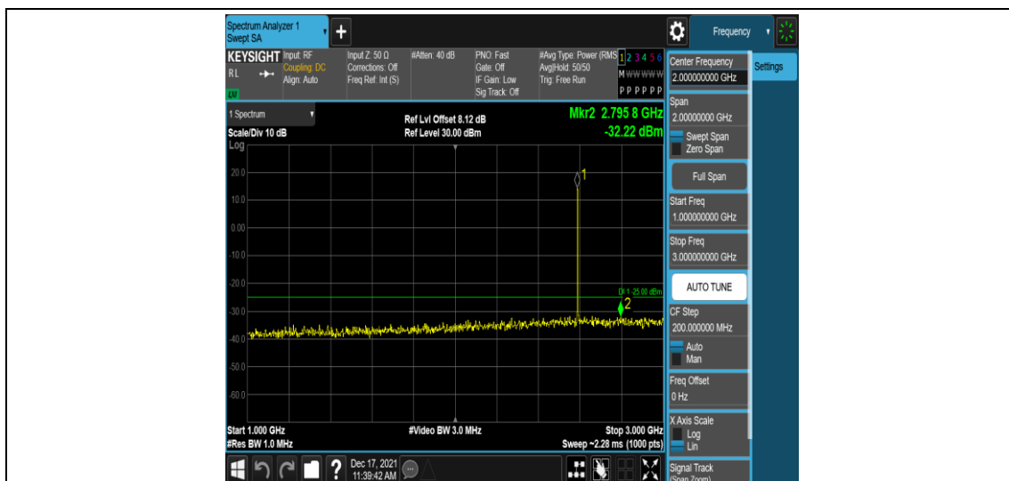
Band41-10MHz-16QAM-40620-1RB#0-Range4:1000~3000MHz
