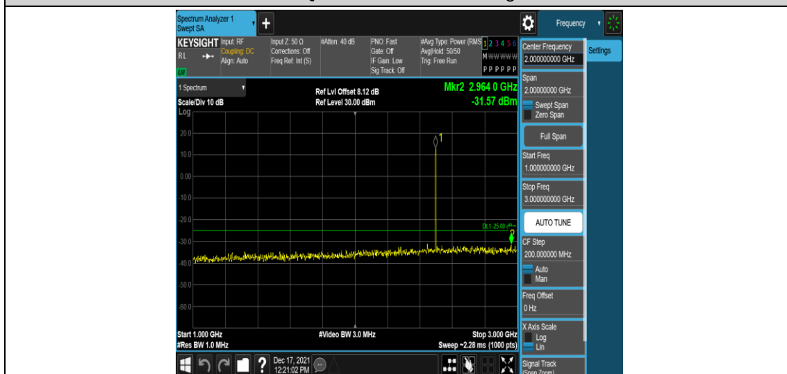
Band41-20MHz-16QAM-39750-1RB#0-Range4:1000~3000MHz
