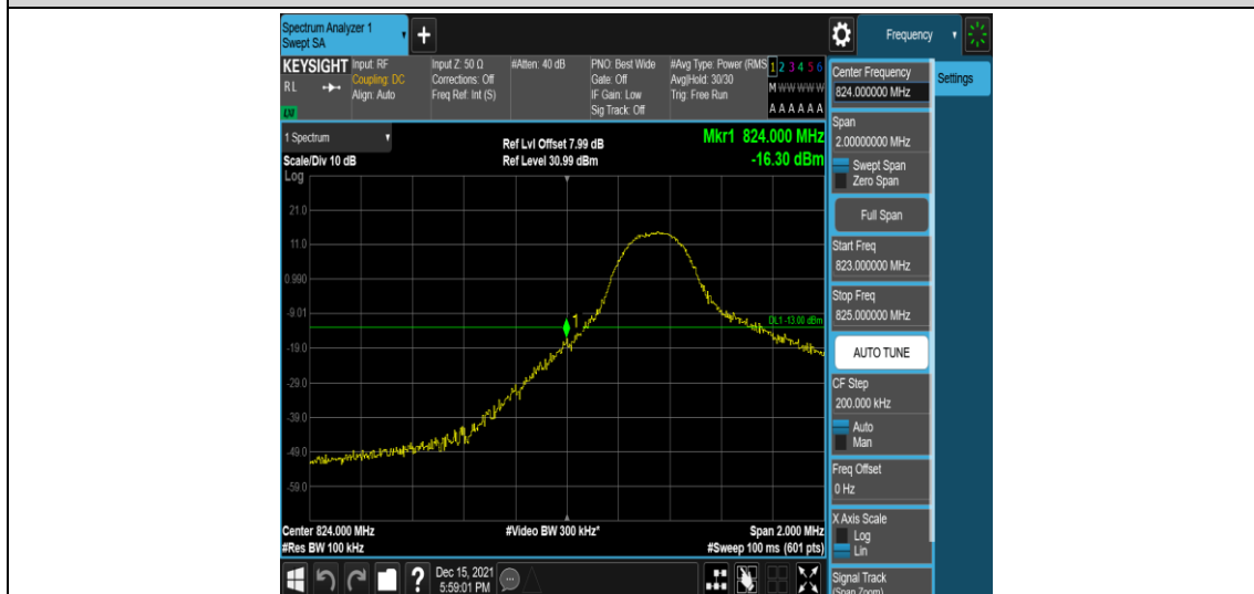
Band5-5MHz-16QAM-20425-1RB#0
