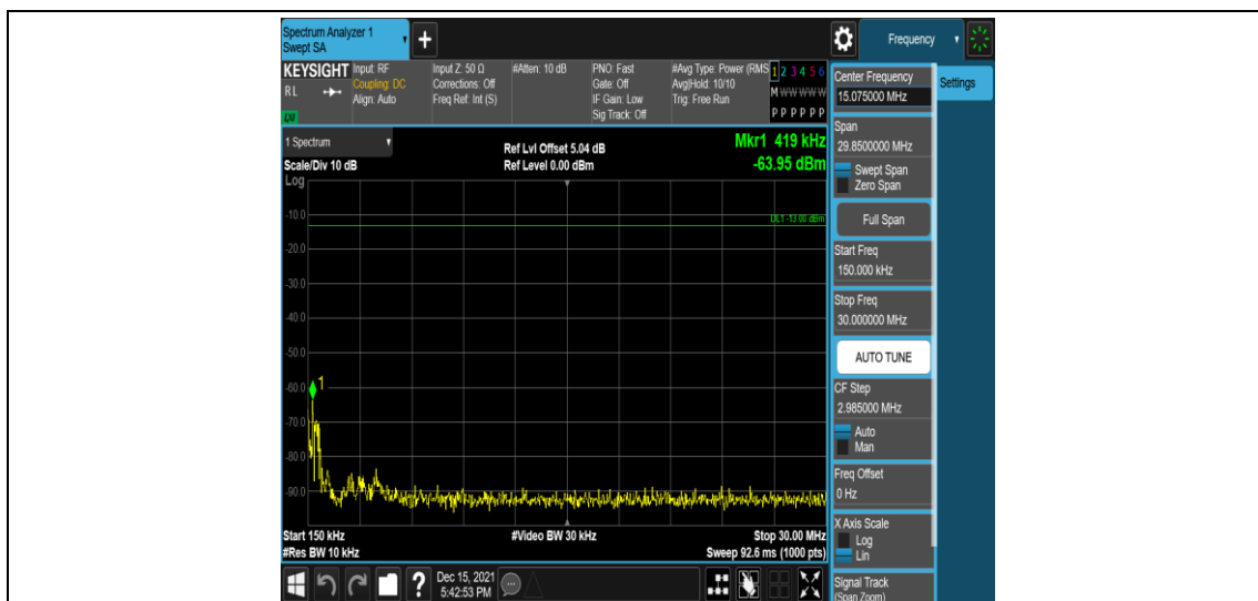
Band5-3MHz-16QAM-20415-1RB#0-Range2:0.15~30MHz
