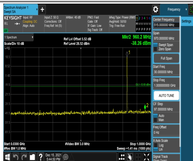
Band5-3MHz-16QAM-20525-1RB#0-Range3:30~1000MHz
