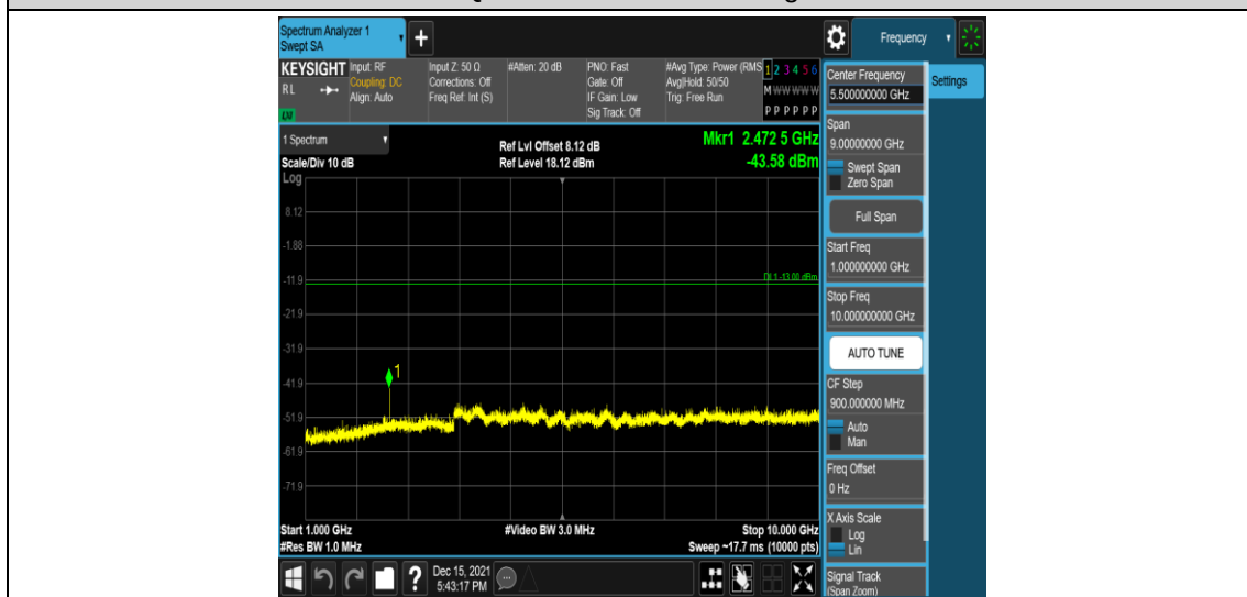
Band5-3MHz-16QAM-20415-1RB#0-Range4:1000~10000MHz
