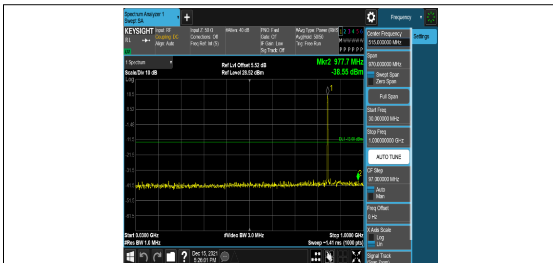
Band5-1.4MHz-QPSK-20643-1RB#0-Range3:30~1000MHz
