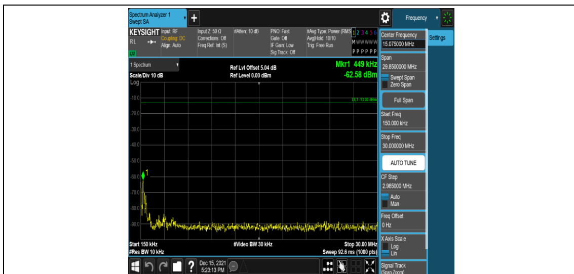
Band5-1.4MHz-16QAM-20407-1RB#0-Range2:0.15~30MHz
