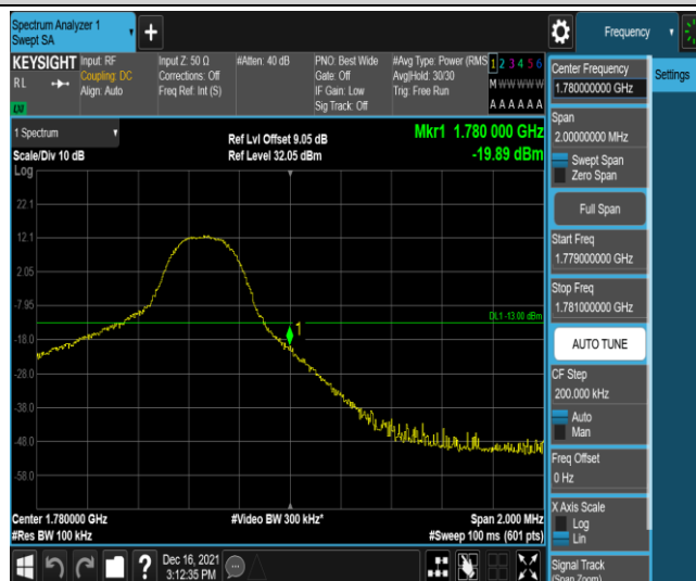
Band66-5MHz-QPSK-132647-1RB#24
