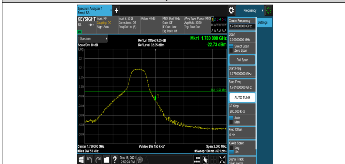
Band66-3MHz-QPSK-132657-1RB#14
