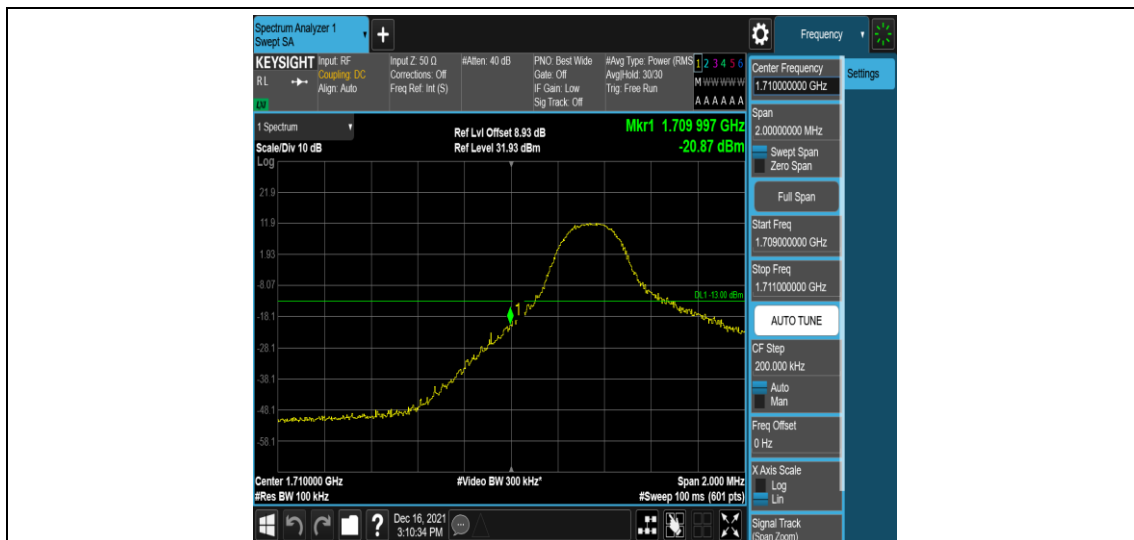
Band66-5MHz-16QAM-131997-1RB#0
