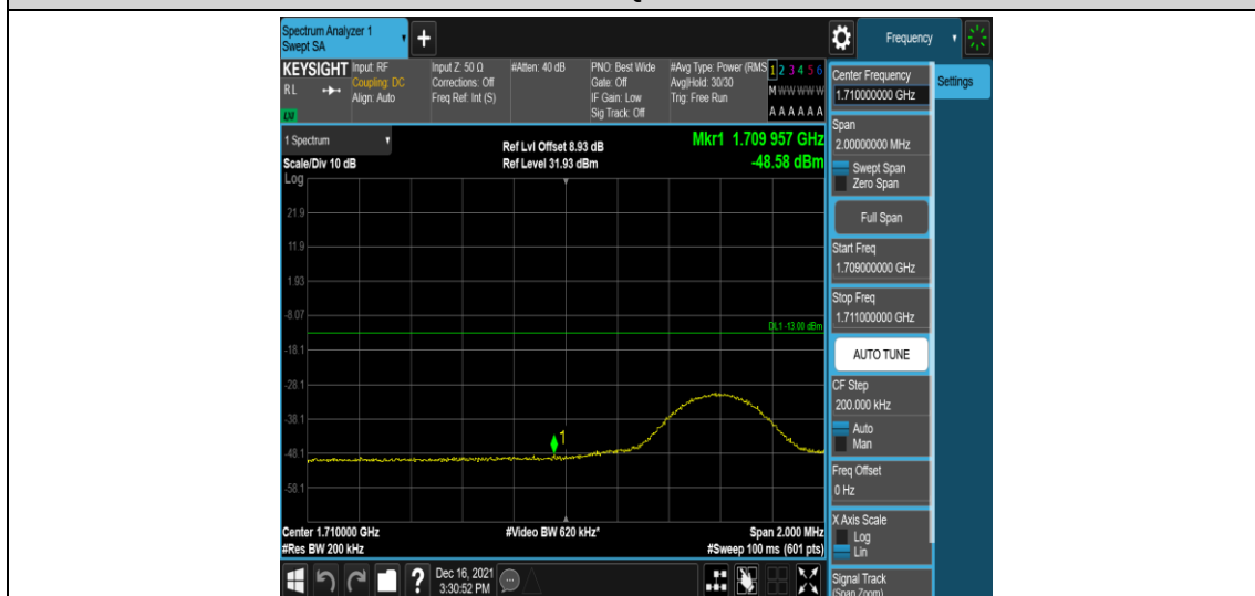
Band66-10MHz-16QAM-132022-1RB#49
