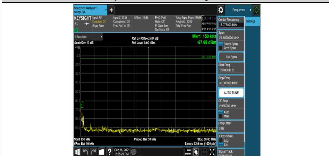
Band66-3MHz-QPSK-132322-1RB#0-Range2:0.15~30MHz
