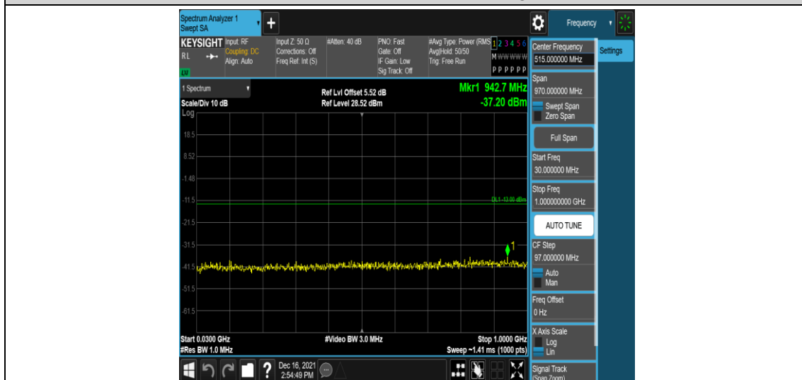
Band66-3MHz-16QAM-131987-1RB#0-Range3:30~1000MHz
