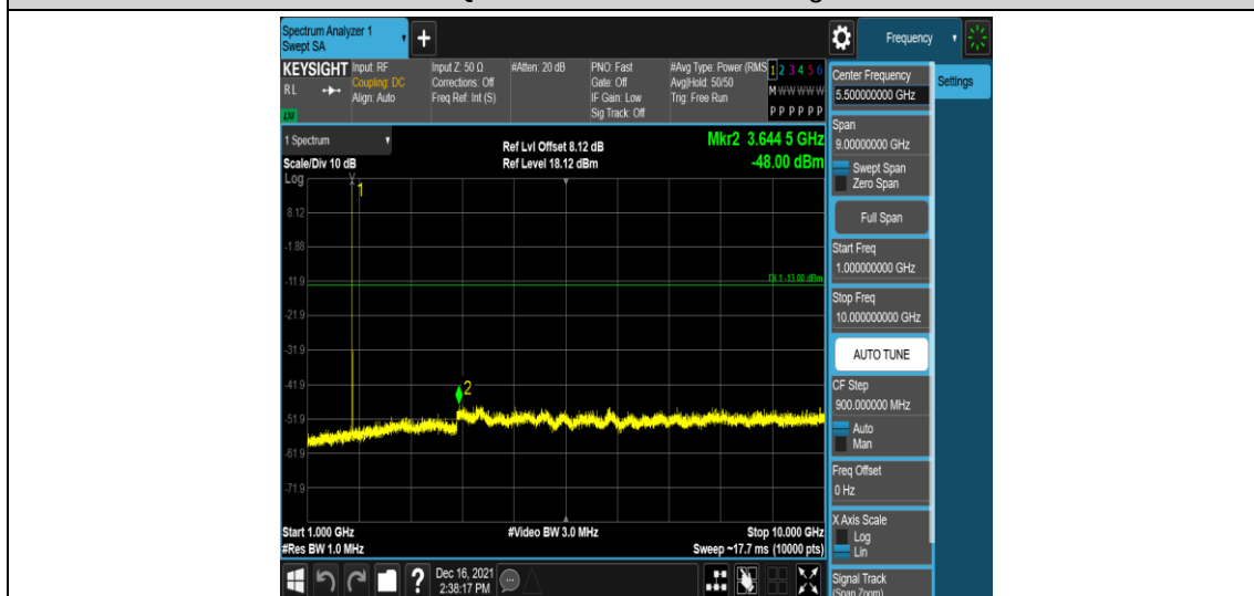
Band66-1.4MHz-QPSK-132665-1RB#0-Range4:1000~10000MHz
