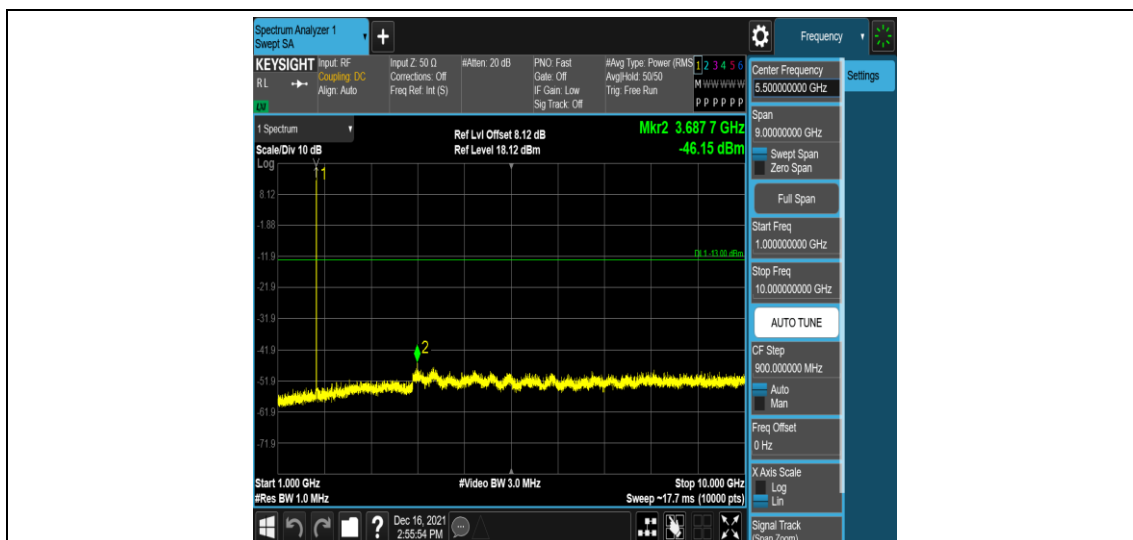
Band66-3MHz-QPSK-132322-1RB#0-Range4:1000~10000MHz
