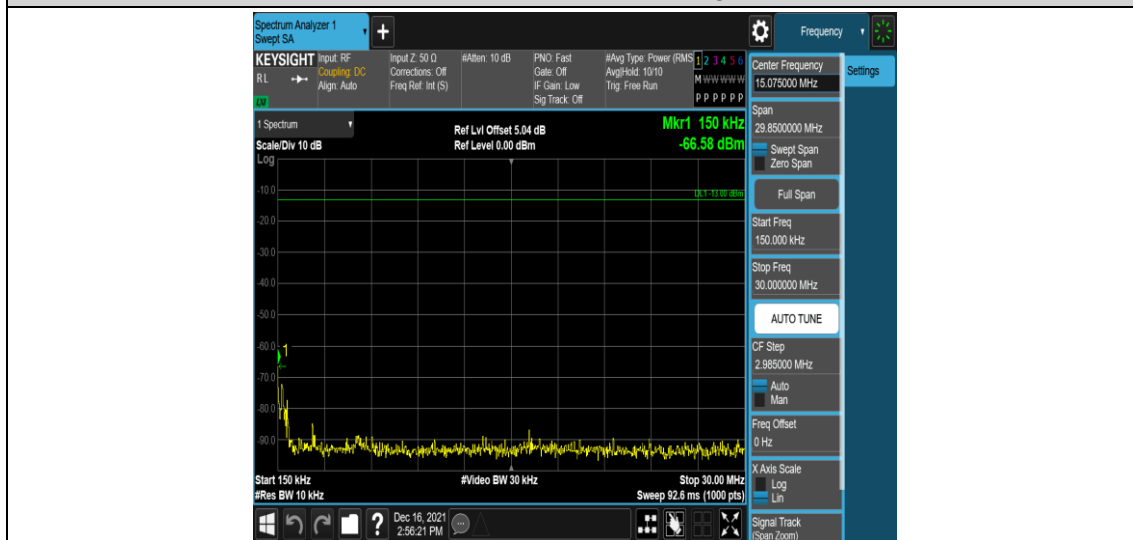
Band66-3MHz-16QAM-132322-1RB#0-Range2:0.15~30MHz
