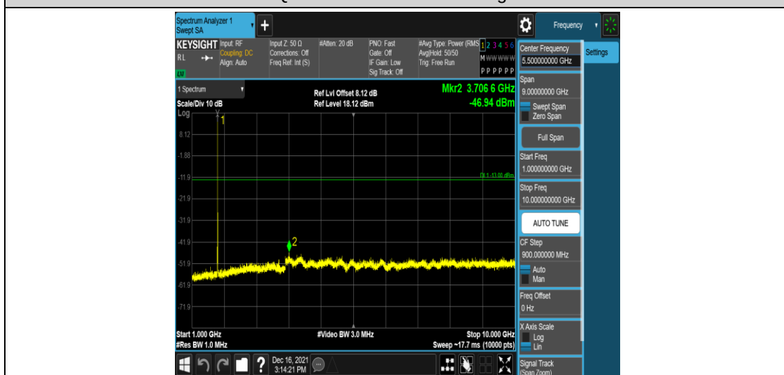
Band66-5MHz-QPSK-131997-1RB#0-Range4:1000~10000MHz
