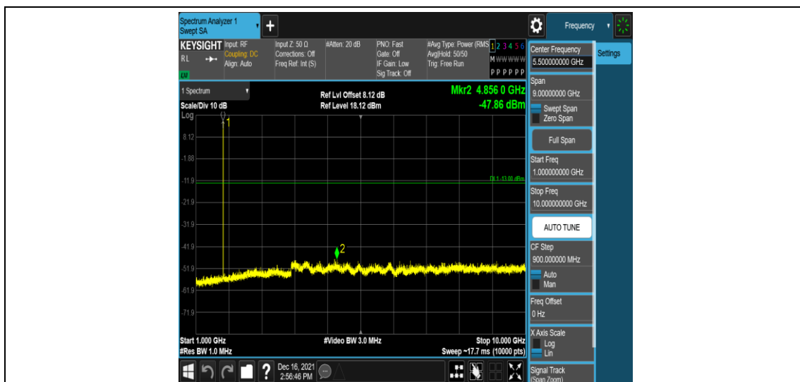
Band66-3MHz-16QAM-132322-1RB#0-Range4:1000~10000MHz
