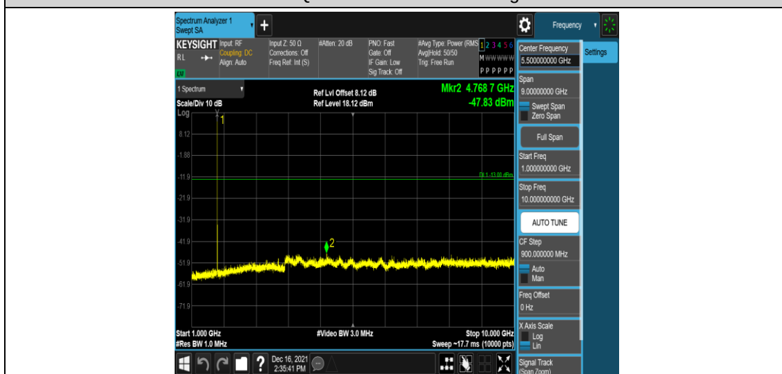
Band66-1.4MHz-16QAM-131979-1RB#0-Range4:1000~10000MHz
