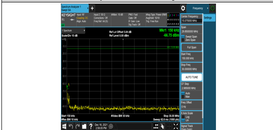
Band66-3MHz-16QAM-132657-1RB#0-Range2:0.15~30MHz
