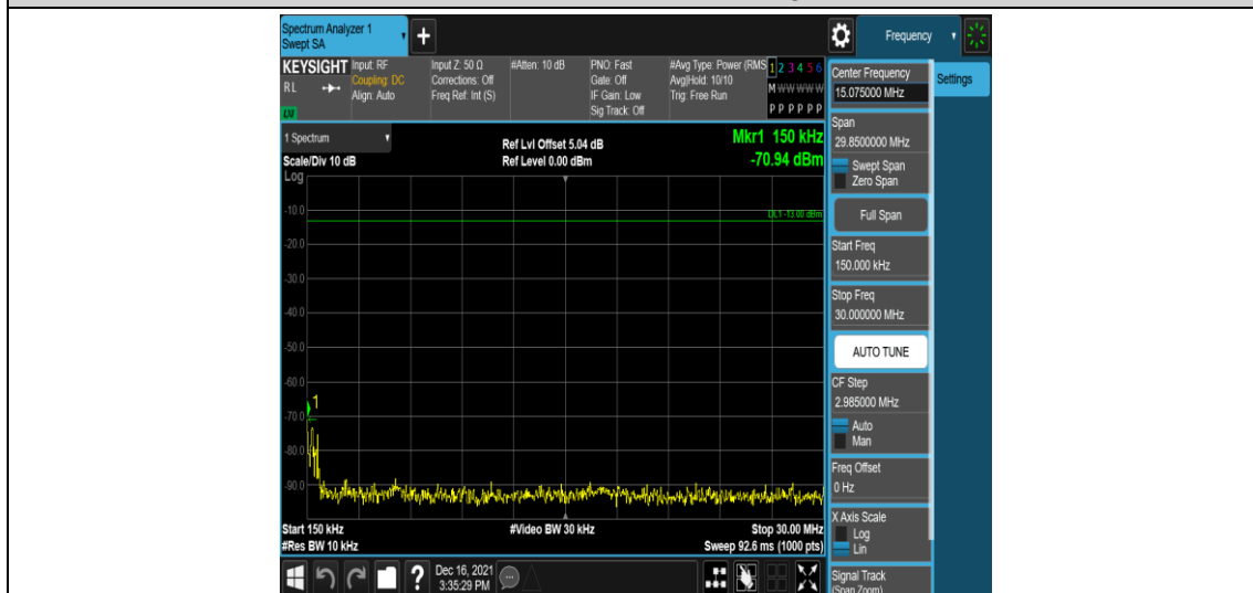
Band66-10MHz-QPSK-132322-1RB#0-Range2:0.15~30MHz
