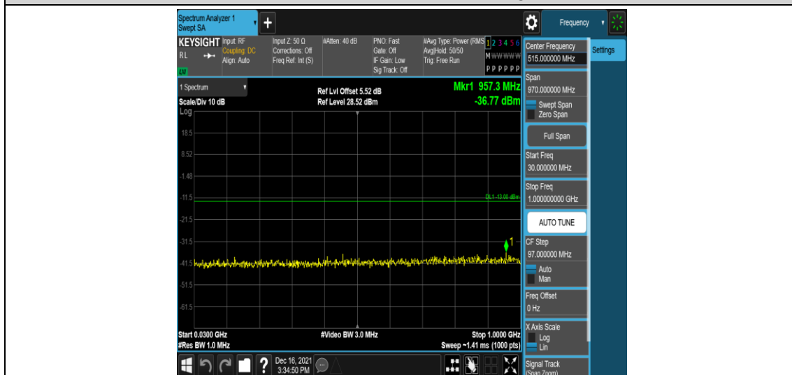
Band66-10MHz-16QAM-132022-1RB#0-Range3:30~1000MHz
