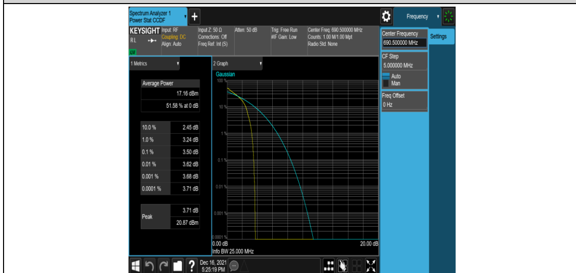
Band71-15MHz-QPSK-133397-1RB#0
