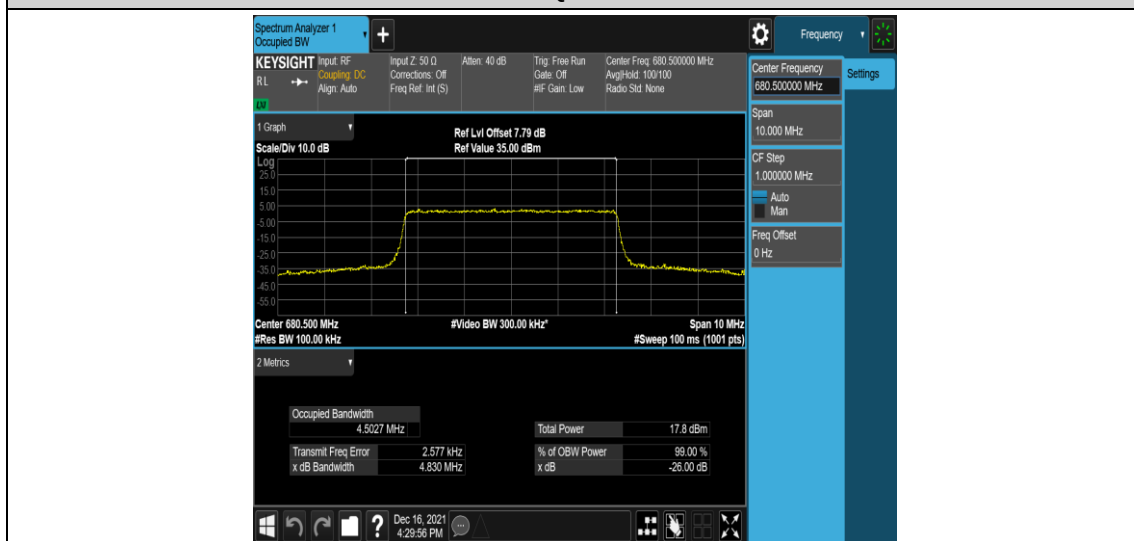
Band71-5MHz-16QAM-133297-25RB#0
