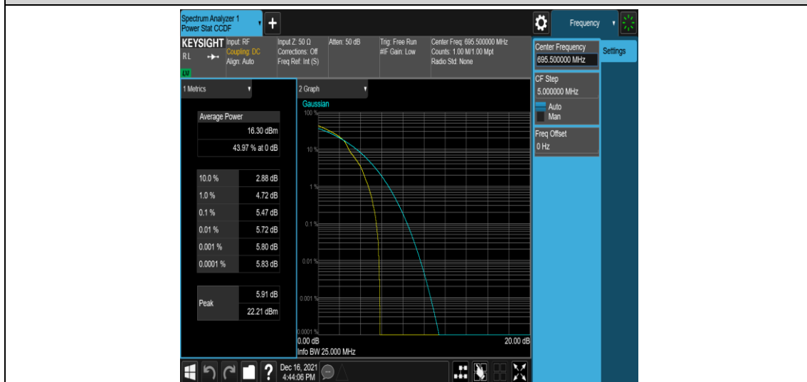
Band71-5MHz-16QAM-133447-1RB#0
