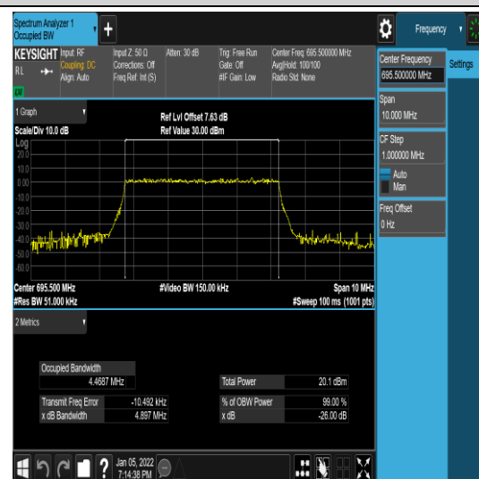
1-N71-PC3-15-5-H-6-CP-16QAM-Outer_Full- 25@0-Ant1-4.4687-4.897-≤5-PASS
