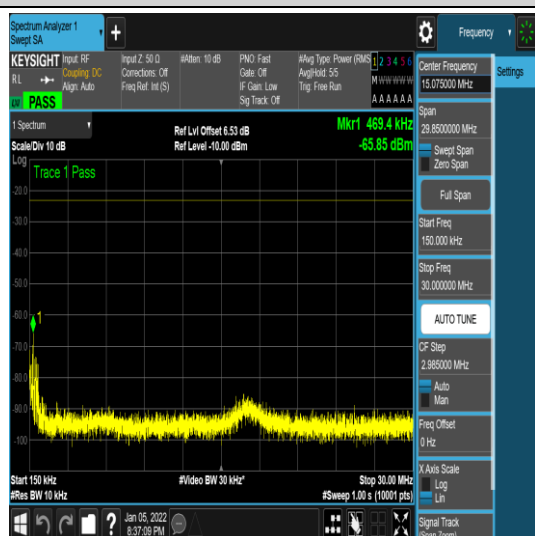
1-N71-PC3-15-15-M-16-CP-QPSK-Edge_1R B_Left-1@0-0.15-30--65.85--23-PASS
