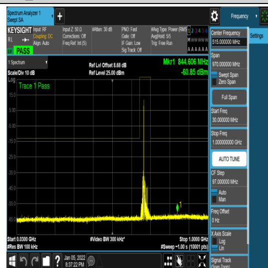
1-N71-PC3-15-15-M-16-CP-QPSK-Edge_1R B_Left-1@0-30-1000--60.85--13-PASS
