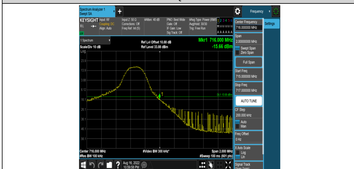
Band12-5MHz-16QAM-23155-1RB#24
