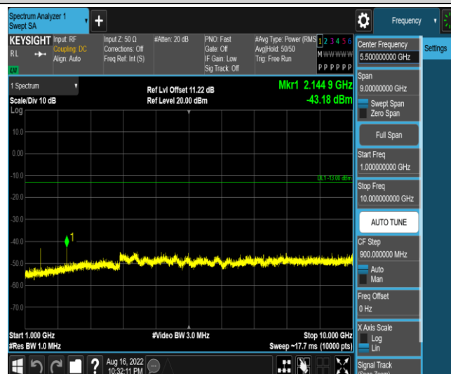
Band12-1.4MHz-QPSK-23173-1RB#0-Range4:1000~10000MHz
