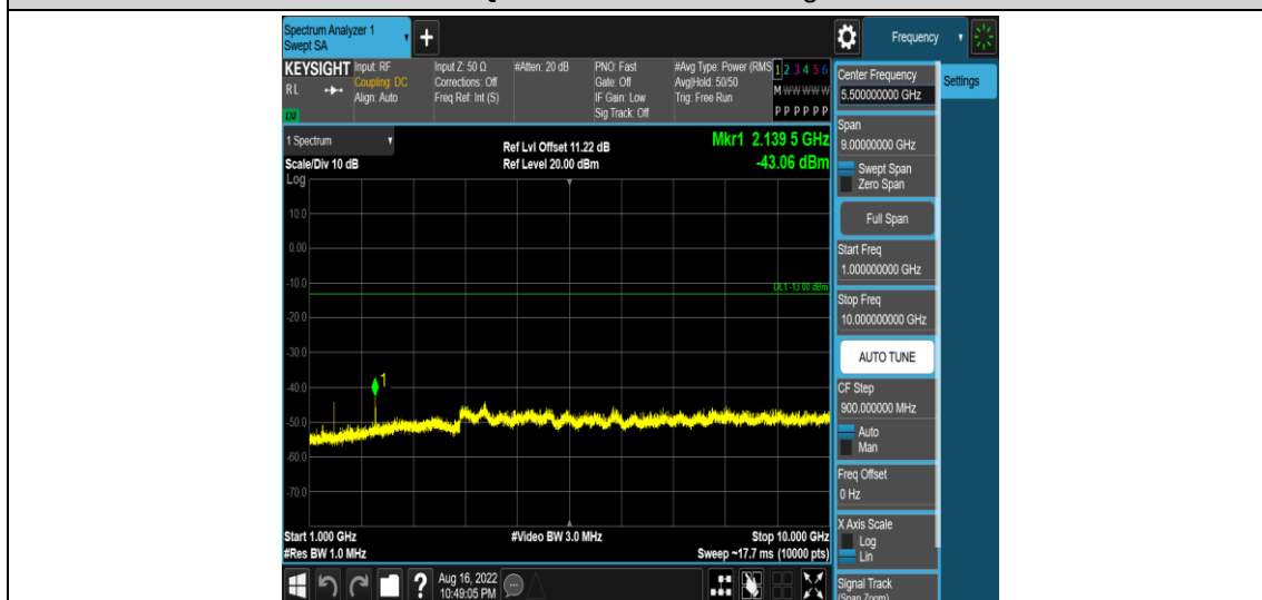
Band12-3MHz-16QAM-23165-1RB#0-Range4:1000~10000MHz
