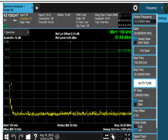
Band12-3MHz-16QAM-23025-1RB#0-Range2:0.15~30MHz
