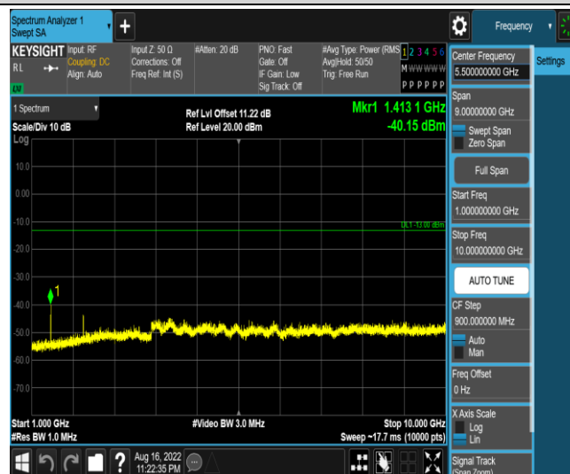
Band12-10MHz-QPSK-23130-1RB#0-Range4:1000~10000MHz
