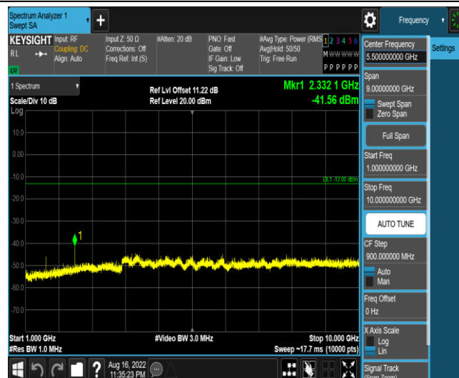
Band13-5MHz-QPSK-23205-1RB#0-Range4:1000~10000MHz
