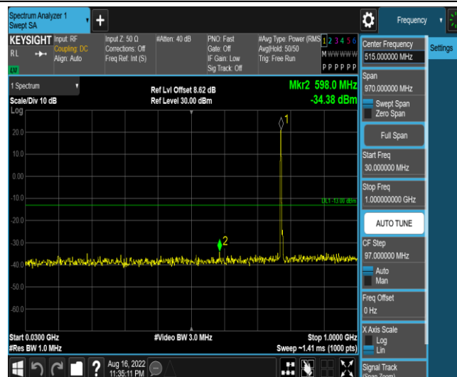
Band13-5MHz-QPSK-23205-1RB#0-Range3:30~1000MHz
