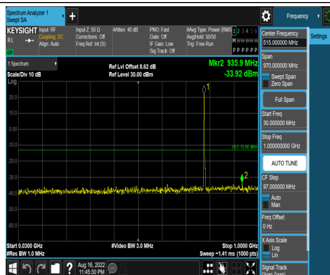
Band13-5MHz-QPSK-23255-1RB#0-Range3:30~1000MHz
