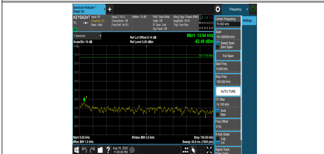
Band13-5MHz-QPSK-23255-1RB#0-Range1:0.009~0.15MHz
