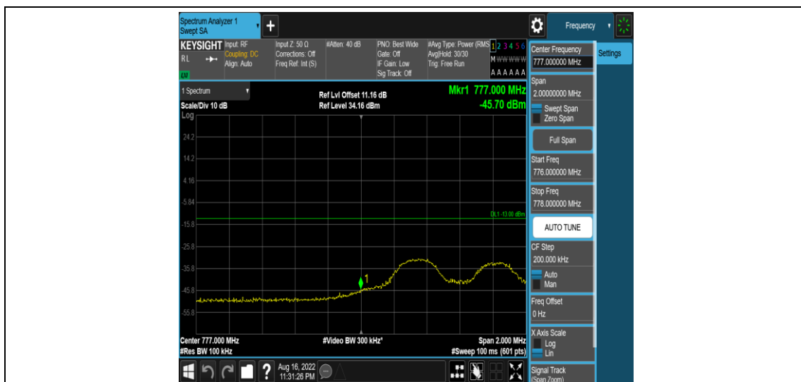
Band13-5MHz-QPSK-23205-1RB#24
