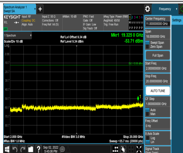
Band2-1.4MHz-QPSK-18900-1RB#0-Range5:2000~20000MHz
