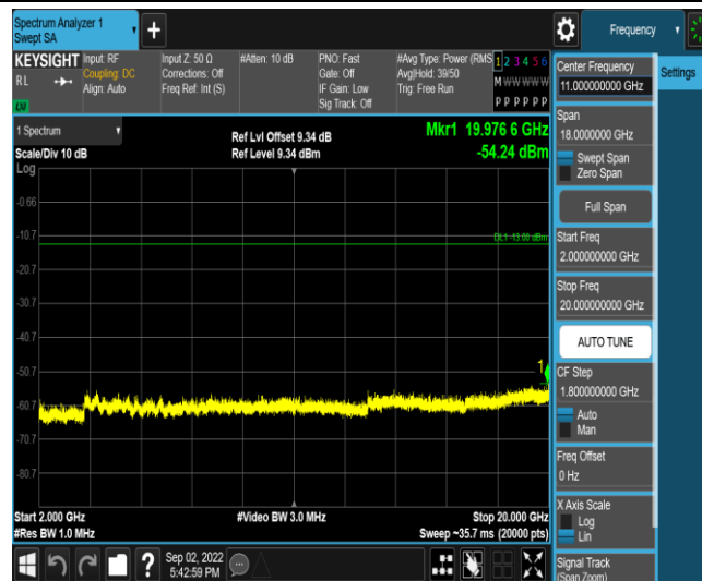
Band2-1.4MHz-QPSK-18607-1RB#0-Range5:2000~20000MHz
