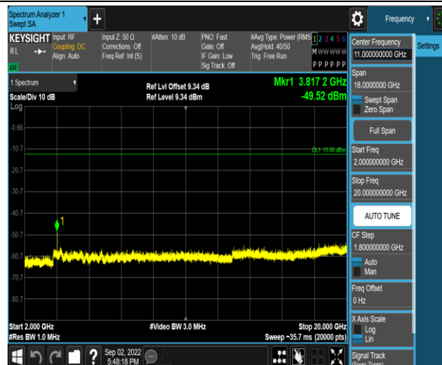
Band2-1.4MHz-16QAM-19193-1RB#0-Range5:2000~20000MHz
