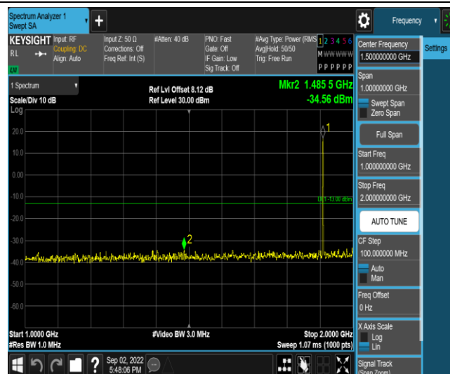
Band2-1.4MHz-16QAM-19193-1RB#0-Range4:1000~2000MHz
