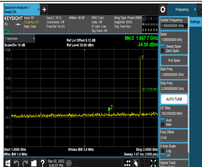
Band2-1.4MHz-16QAM-18900-1RB#0-Range4:1000~2000MHz
