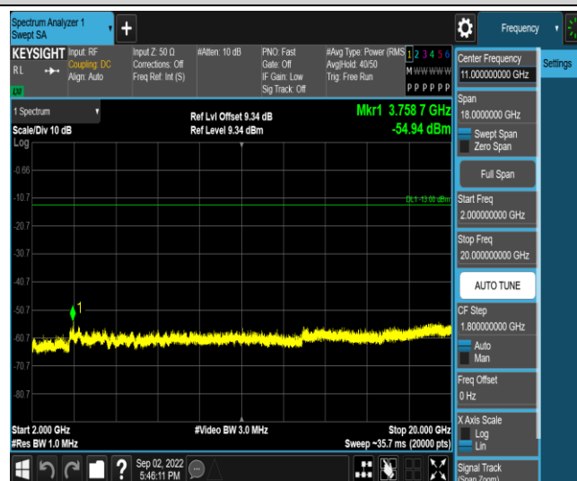
Band2-1.4MHz-16QAM-18900-1RB#0-Range5:2000~20000MHz
