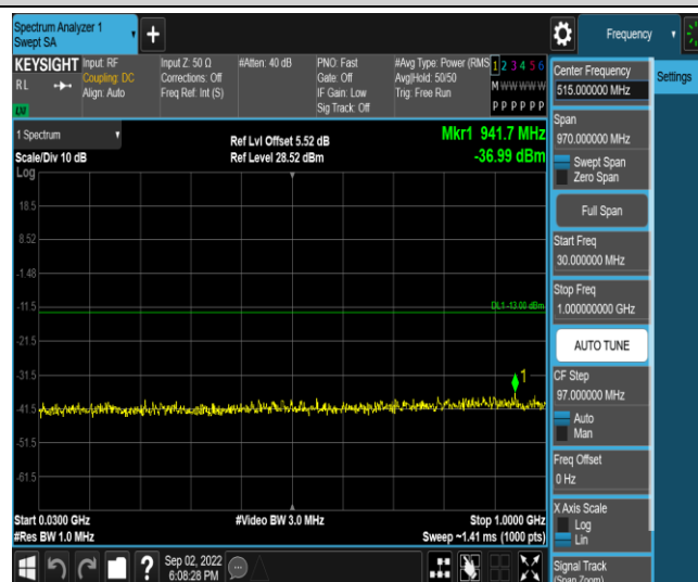
Band2-3MHz-16QAM-19185-1RB#0-Range3:30~1000MHz
