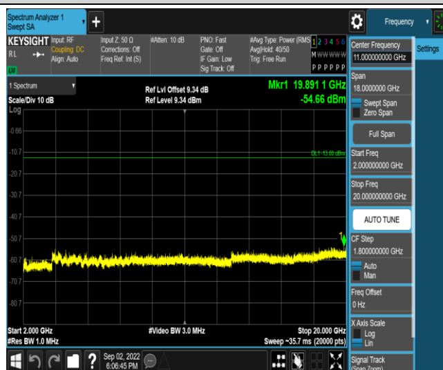
Band2-3MHz-16QAM-18900-1RB#0-Range5:2000~20000MHz
