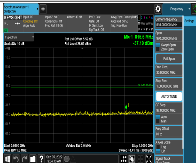
Band2-10MHz-16QAM-19150-1RB#0-Range3:30~1000MHz
