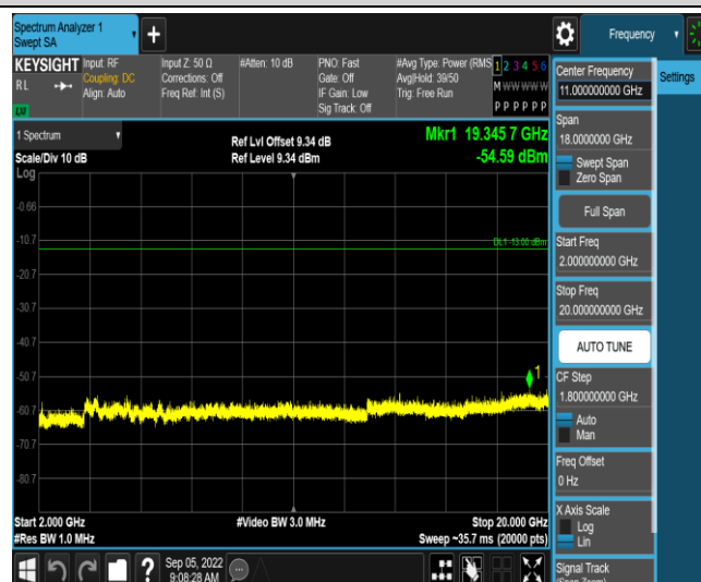
Band2-5MHz-16QAM-18900-1RB#0-Range5:2000~20000MHz
