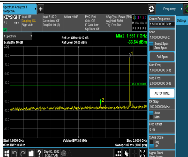
Band2-10MHz-16QAM-18900-1RB#0-Range4:1000~2000MHz
