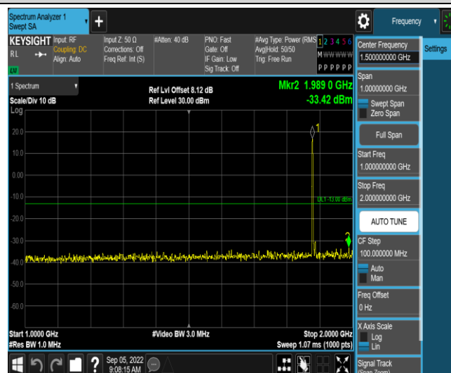
Band2-5MHz-16QAM-18900-1RB#0-Range4:1000~2000MHz
