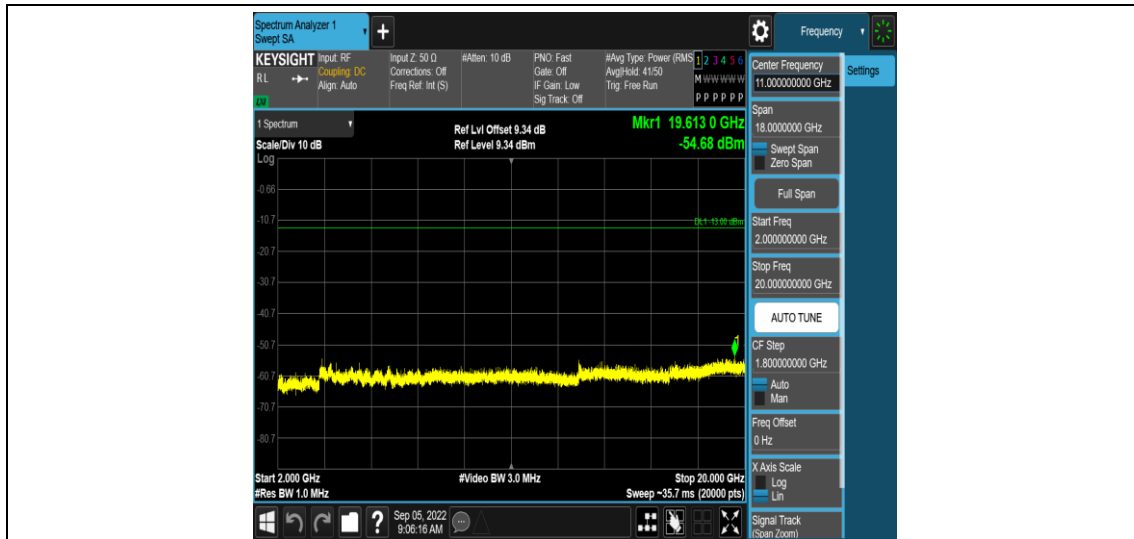
Band2-5MHz-16QAM-18625-1RB#0-Range5:2000~20000MHz
