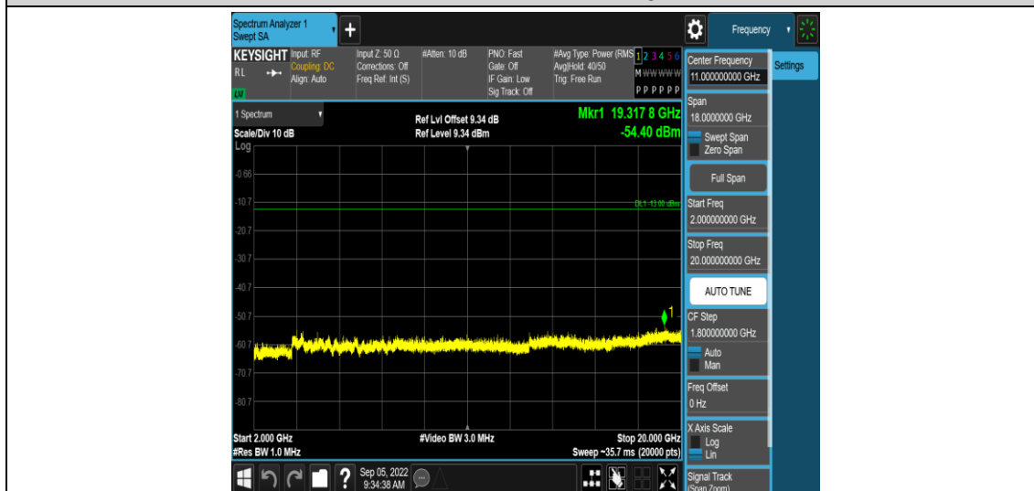
Band2-10MHz-16QAM-19150-1RB#0-Range5:2000~20000MHz
