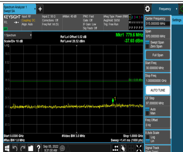
Band2-10MHz-QPSK-18900-1RB#0-Range3:30~1000MHz
