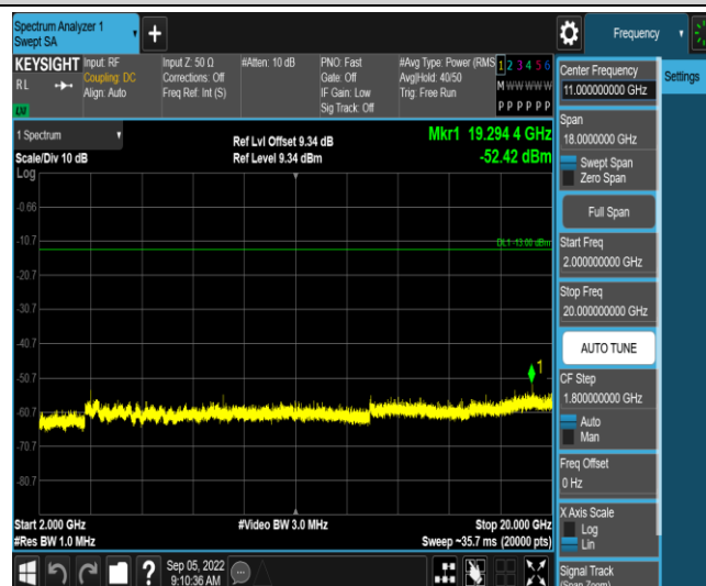
Band2-5MHz-16QAM-19175-1RB#0-Range5:2000~20000MHz
