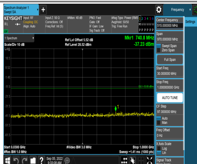
Band2-10MHz-QPSK-19150-1RB#0-Range3:30~1000MHz
