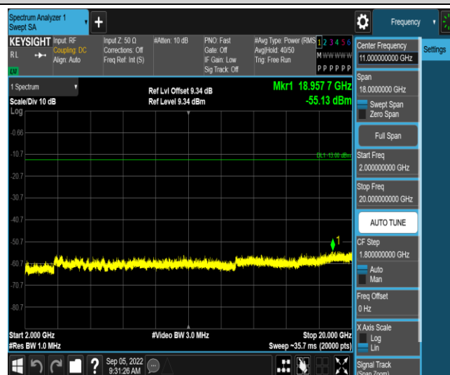
Band2-10MHz-QPSK-18900-1RB#0-Range5:2000~20000MHz
