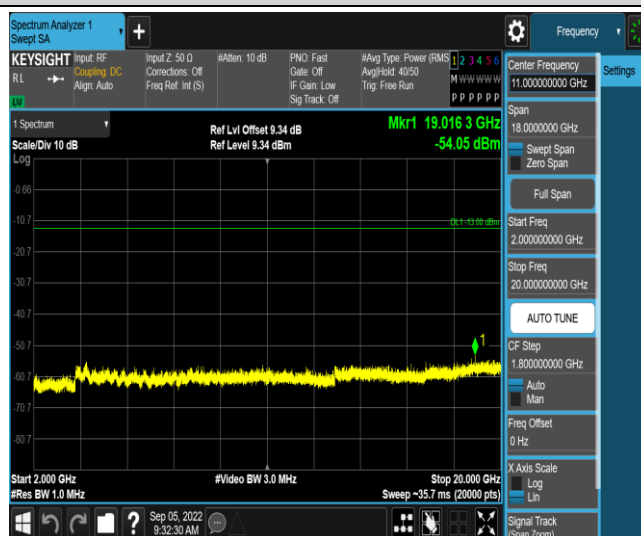
Band2-10MHz-16QAM-18900-1RB#0-Range5:2000~20000MHz
