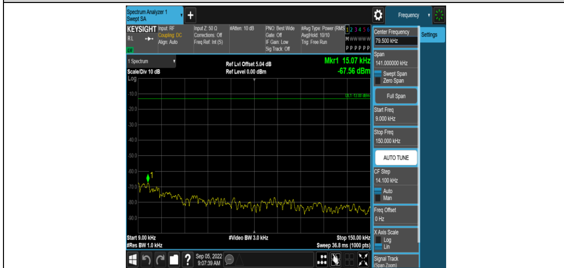
Band2-5MHz-16QAM-18900-1RB#0-Range1:0.009~0.15MHz
