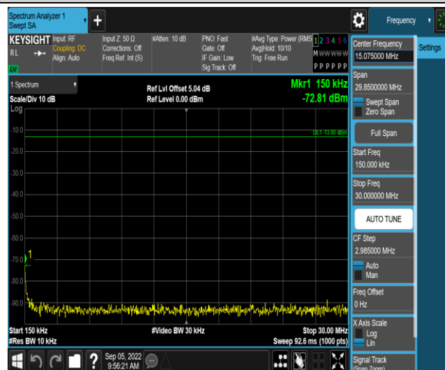
Band2-15MHz-16QAM-18900-1RB#0-Range2:0.15~30MHz
