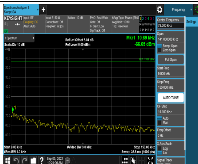
Band2-20MHz-16QAM-19100-1RB#0-Range1:0.009~0.15MHz
