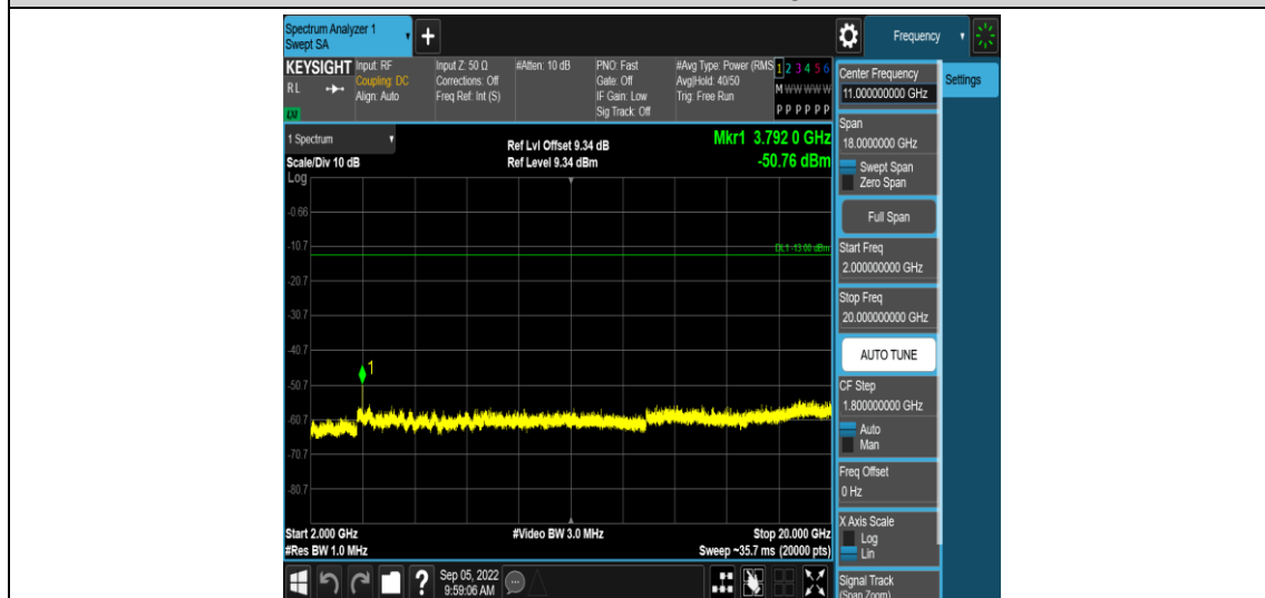
Band2-15MHz-16QAM-19125-1RB#0-Range5:2000~20000MHz
