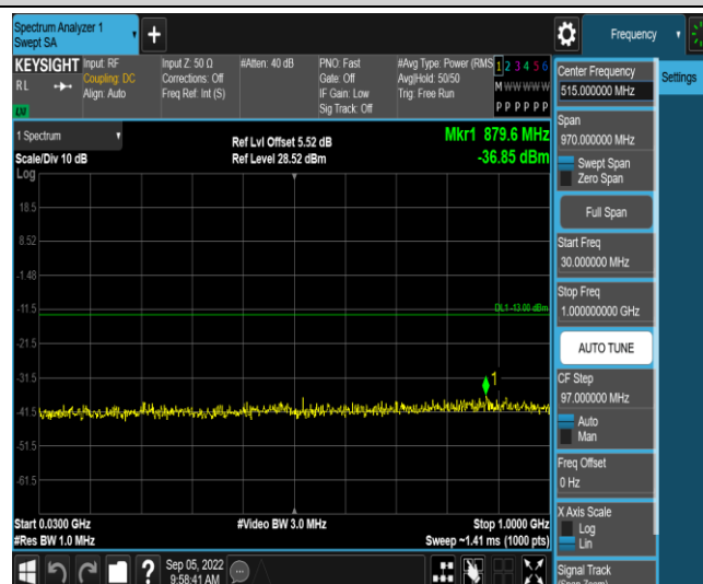
Band2-15MHz-16QAM-19125-1RB#0-Range3:30~1000MHz
