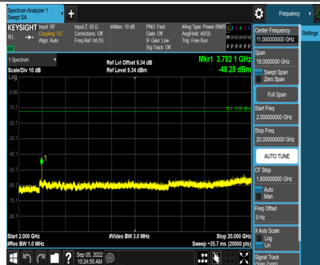
Band2-20MHz-16QAM-19100-1RB#0-Range5:2000~20000MHz
