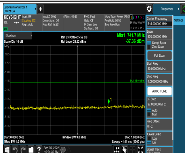
Band2-20MHz-16QAM-19100-1RB#0-Range3:30~1000MHz
