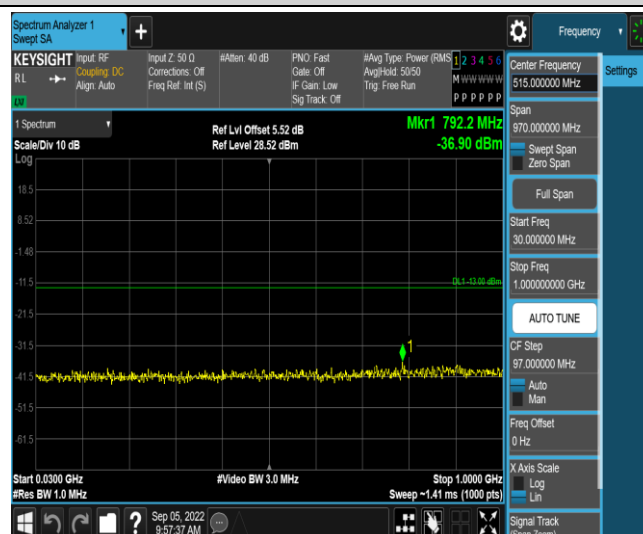
Band2-15MHz-QPSK-19125-1RB#0-Range3:30~1000MHz
