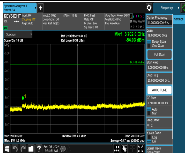
Band2-15MHz-16QAM-18675-1RB#0-Range5:2000~20000MHz
