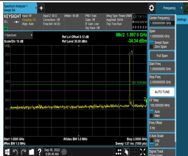
Band2-15MHz-16QAM-18900-1RB#0-Range4:1000~2000MHz
