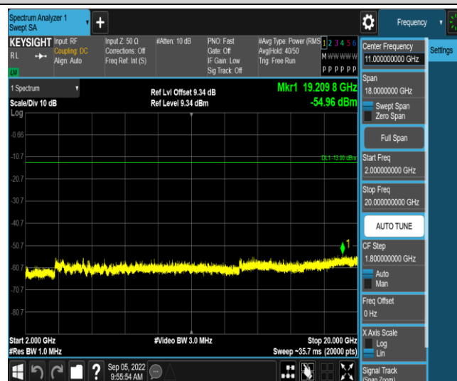
Band2-15MHz-QPSK-18900-1RB#0-Range5:2000~20000MHz
