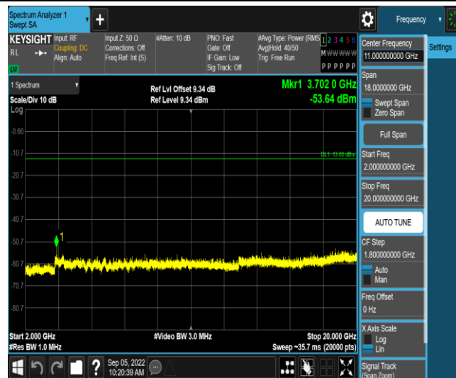
Band2-20MHz-16QAM-18700-1RB#0-Range5:2000~20000MHz
