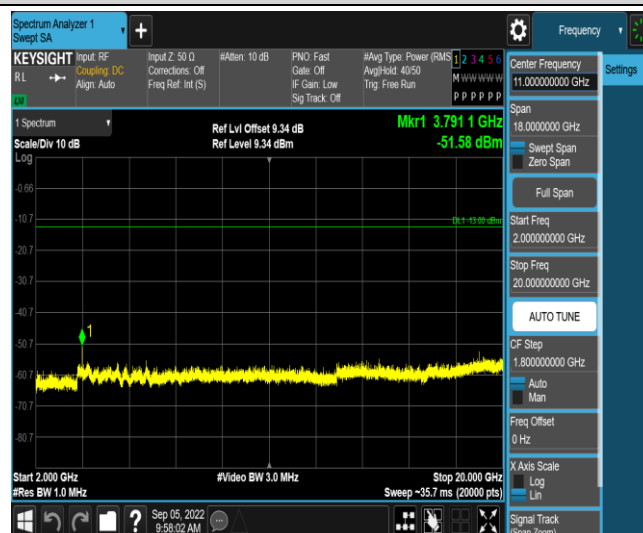
Band2-15MHz-QPSK-19125-1RB#0-Range5:2000~20000MHz
