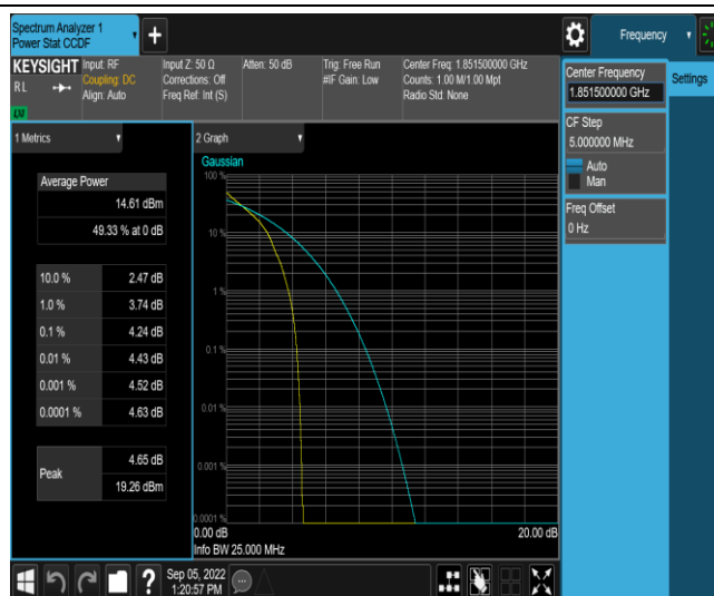
Band25-3MHz-QPSK-26055-1RB#0
