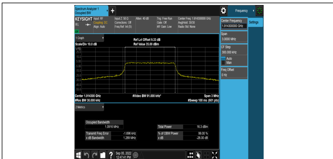
Band25-1.4MHz-QPSK-26683-6RB#0
