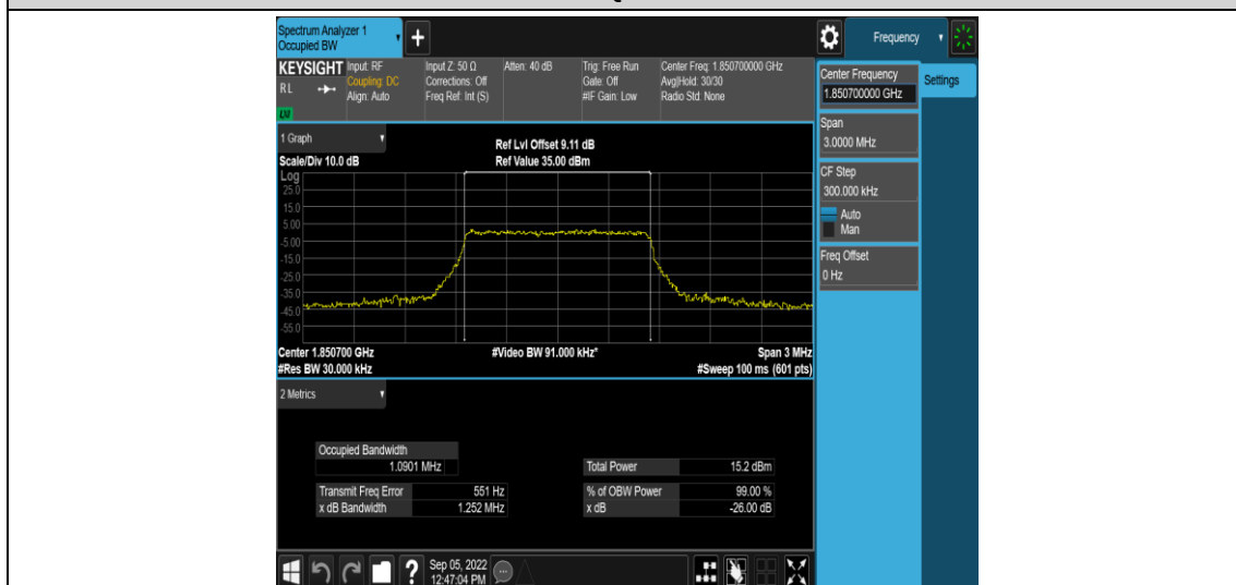
Band25-1.4MHz-16QAM-26047-6RB#0
