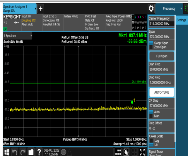
Band25-3MHz-QPSK-26675-1RB#0-Range3:30~1000MHz
