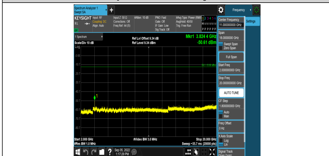
Band25-3MHz-QPSK-26675-1RB#0-Range5:2000~20000MHz
