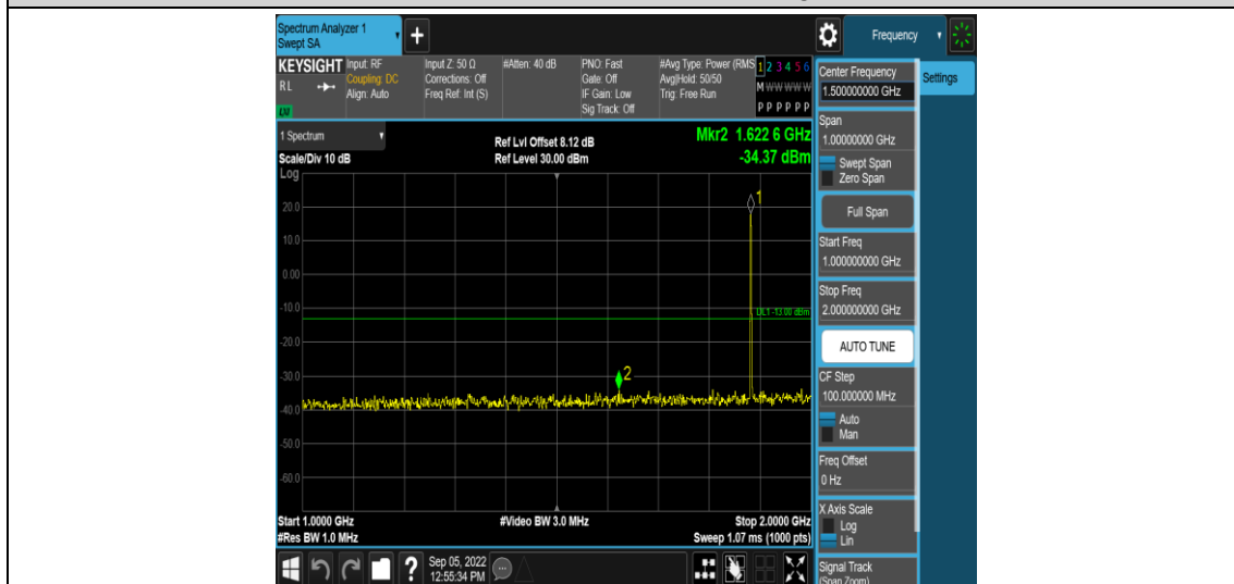
Band25-1.4MHz-16QAM-26365-1RB#0-Range4:1000~2000MHz
