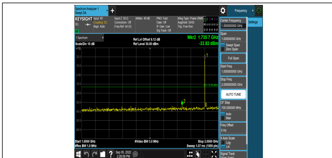
Band25-15MHz-16QAM-26615-1RB#0-Range4:1000~2000MHz
