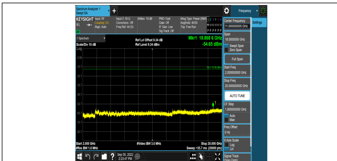
Band25-15MHz-QPSK-26115-1RB#0-Range5:2000~20000MHz
