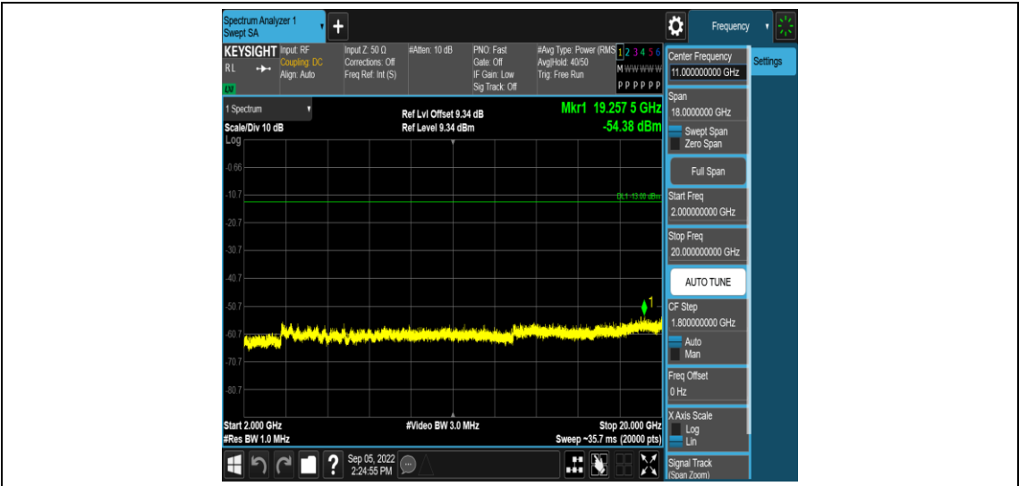
Band25-15MHz-16QAM-26115-1RB#0-Range5:2000~20000MHz
