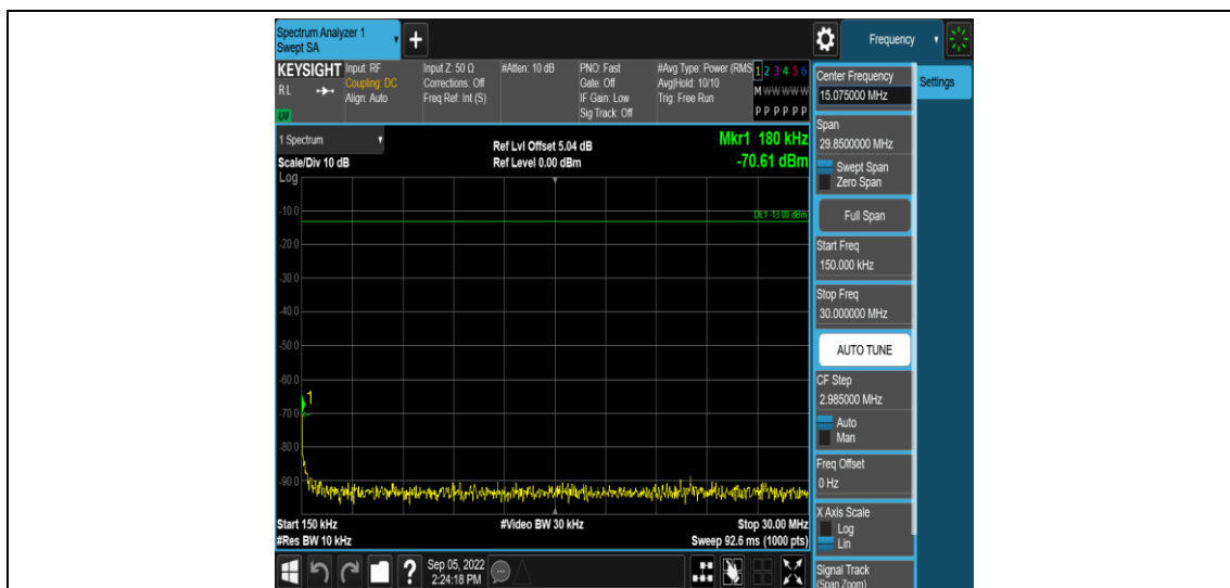
Band25-15MHz-16QAM-26115-1RB#0-Range2:0.15~30MHz
