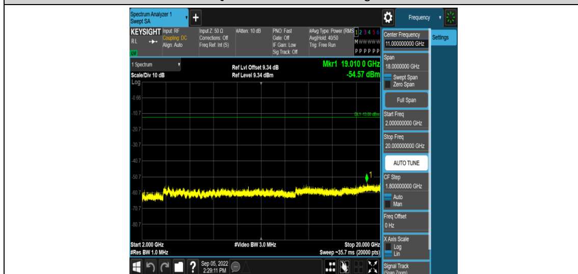
Band25-15MHz-16QAM-26615-1RB#0-Range5:2000~20000MHz
