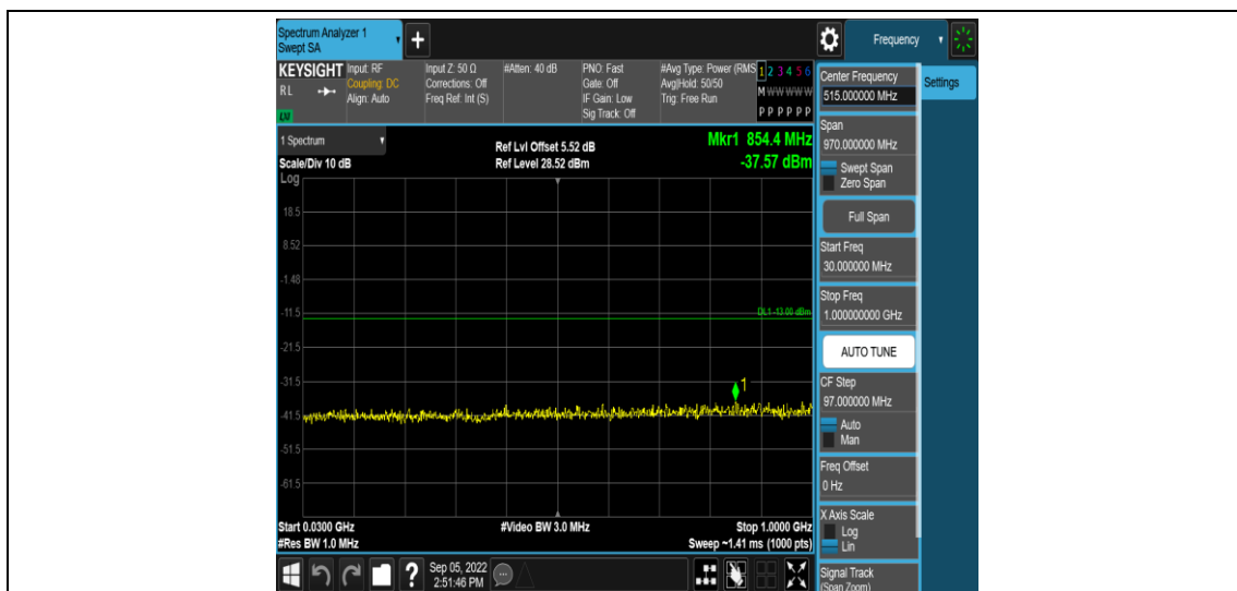
Band25-20MHz-16QAM-26365-1RB#0-Range3:30~1000MHz
