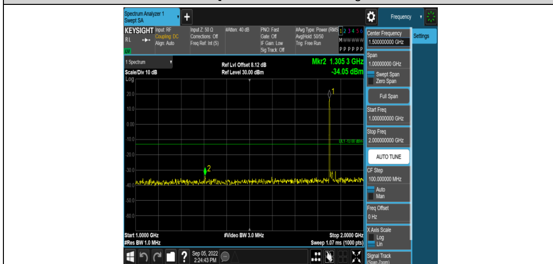
Band25-15MHz-16QAM-26115-1RB#0-Range4:1000~2000MHz
