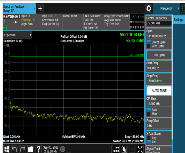
Band25-20MHz-QPSK-26590-1RB#0-Range1:0.009~0.15MHz
