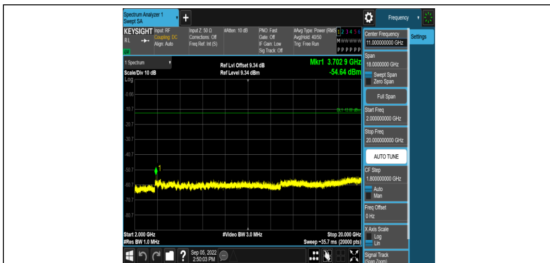
Band25-20MHz-16QAM-26140-1RB#0-Range5:2000~20000MHz
